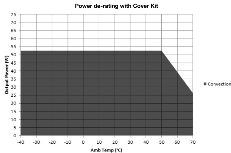
Figure 1. Derating Curves
