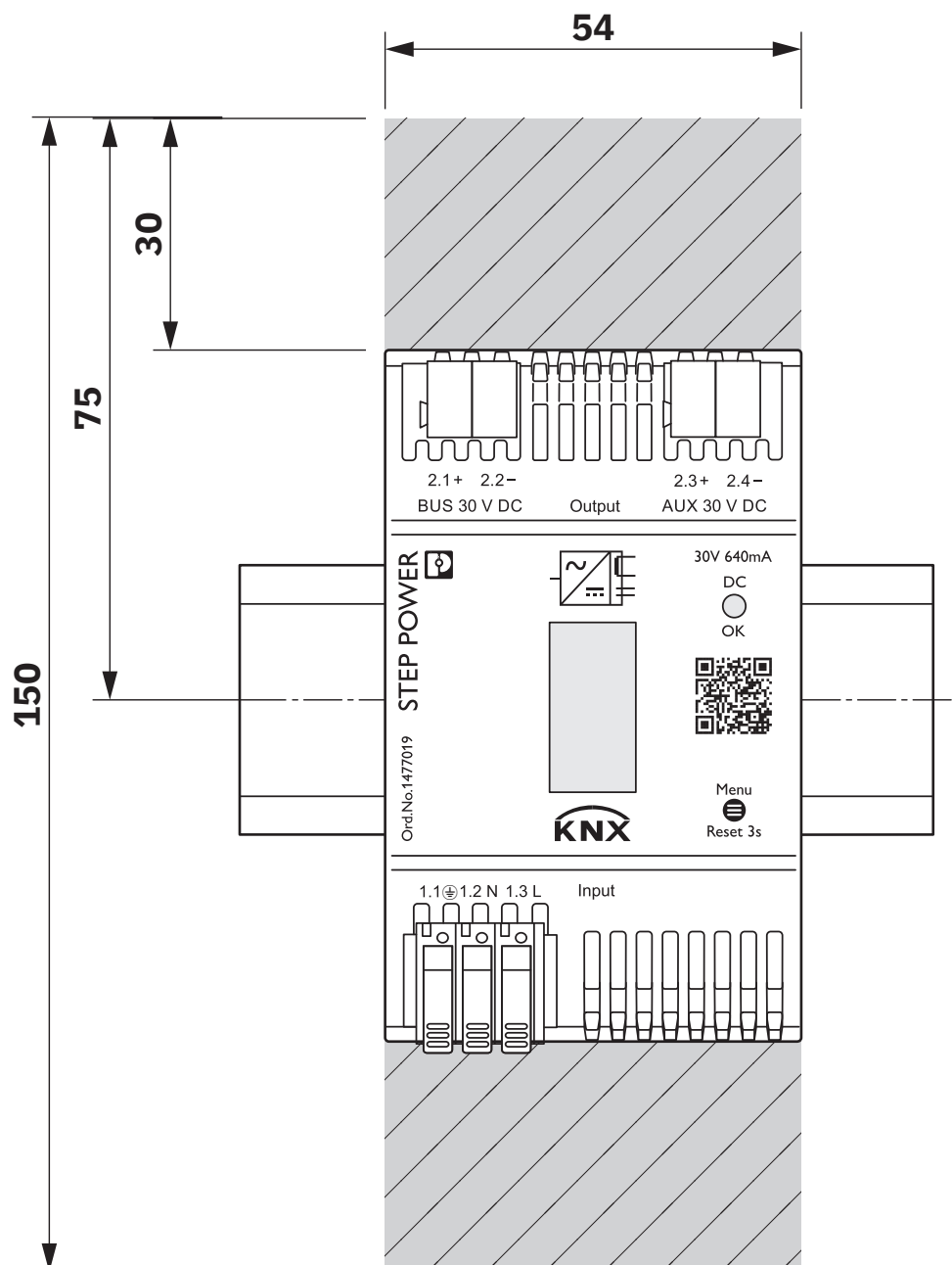
Dimensional drawing
