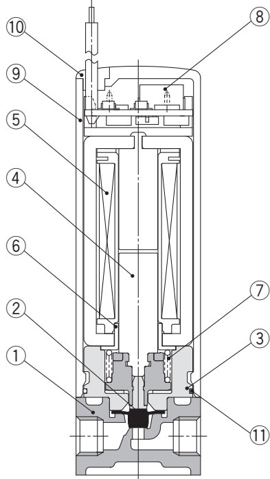
Component Parts: LVM11
