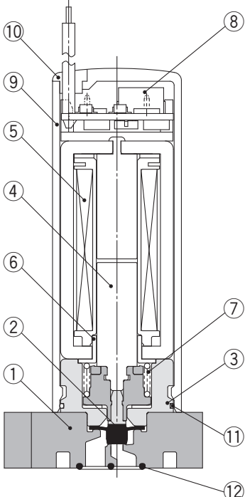
Component Parts: LVM13
