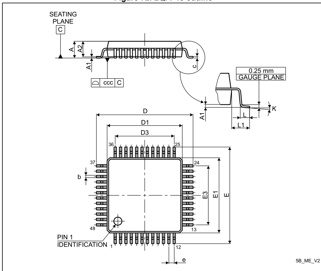
Figure 72. LQFP48 outline
