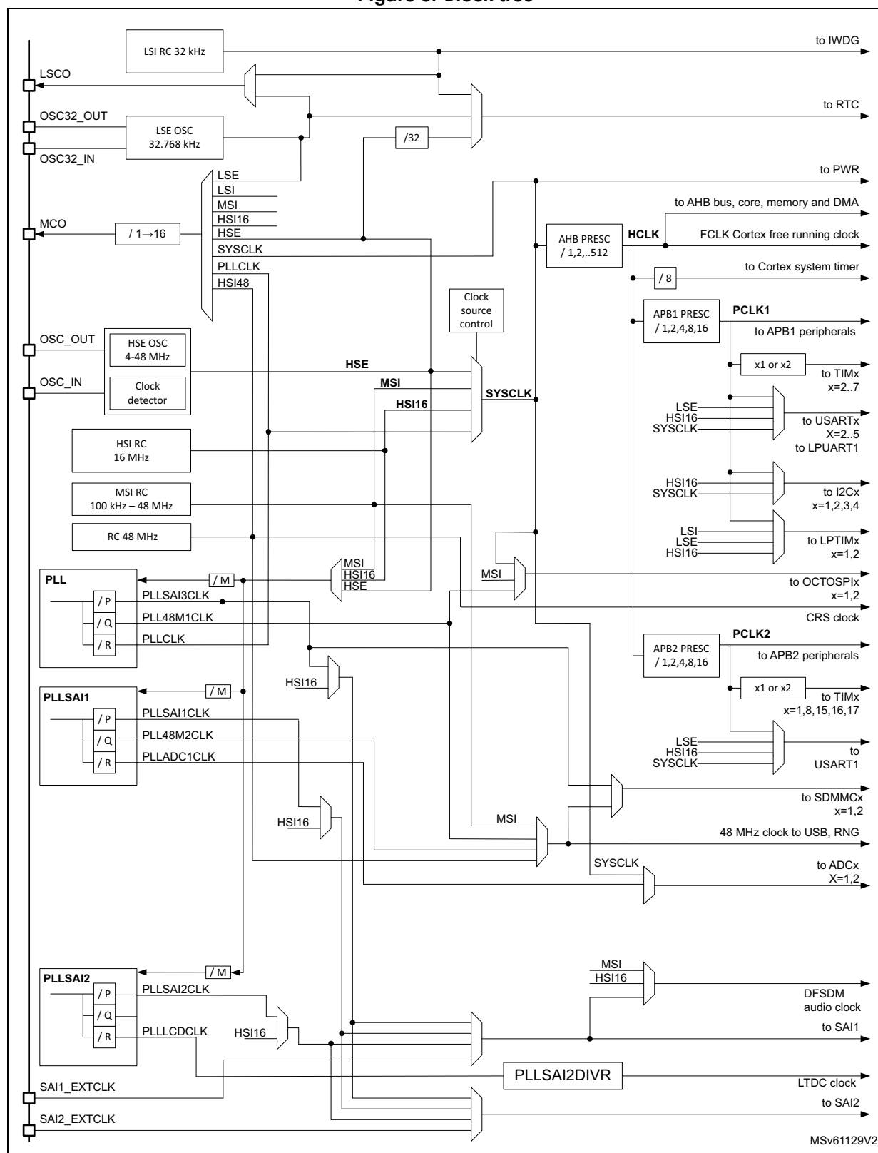
Figure 5. Clock tree
