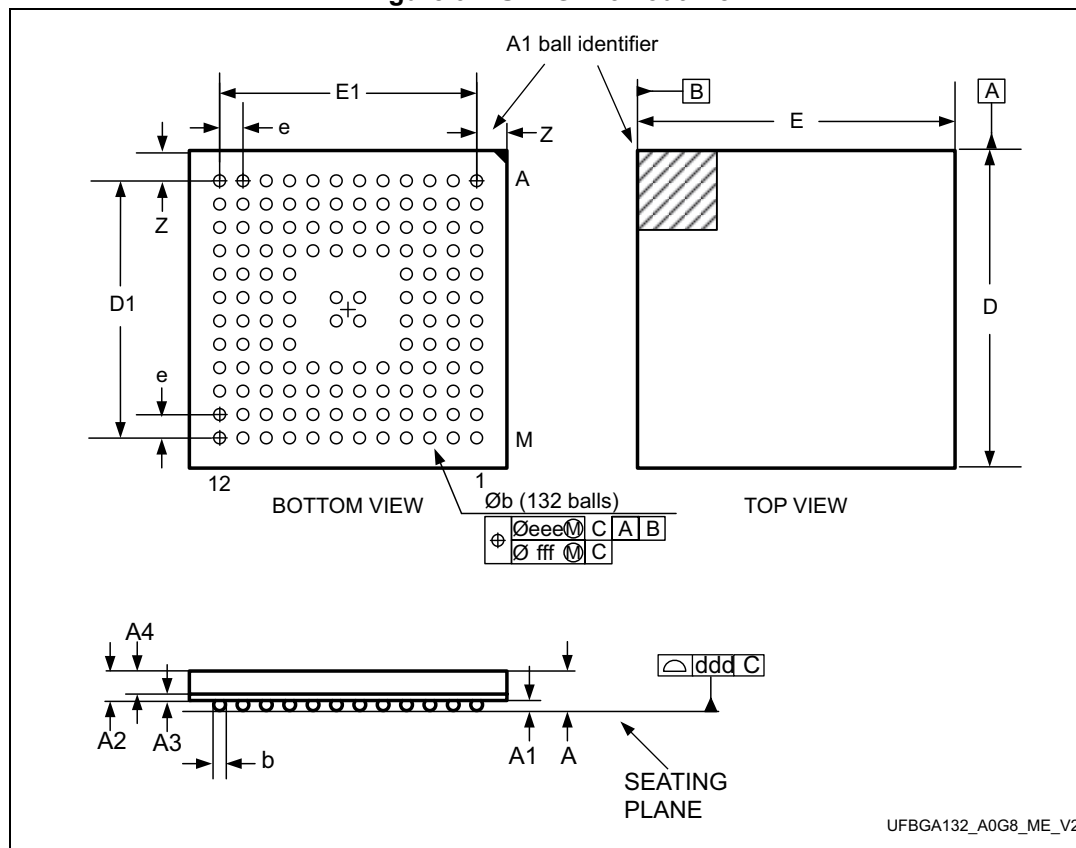
Figure 92. UFBGA132 outline
