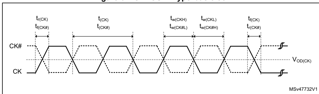
Figure 62. OCTOSPI Hyperbus clock
