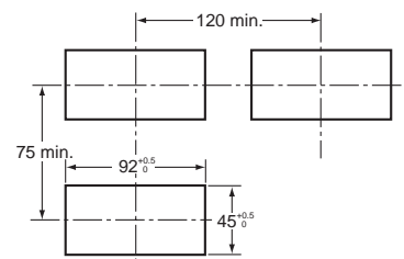
Panel cut-out
