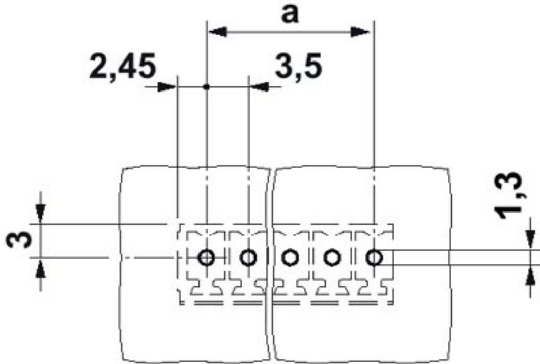
Drilling diagram
