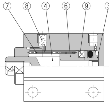
Built-in magnet
