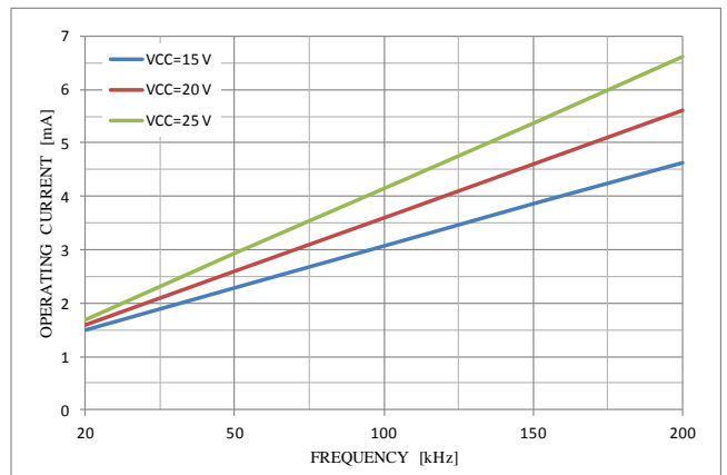
Figure 10. Operating Supply Current vs. Switching Frequency (C LOAD = 1 nF)
