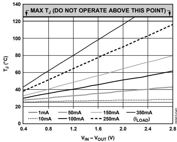
Figure 40. 500 \text{mm}^2 of PCB Copper, T_A = 25^{\circ}\text{C} , TSOT
