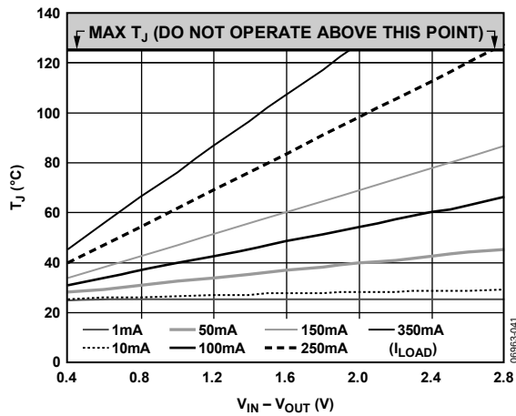
Figure 41. 100 \text{mm}^2 of PCB Copper, T_A = 25^{\circ}\text{C} , TSOT
