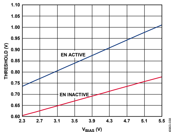
Figure 38. Typical EN Pin Thresholds vs. Input
