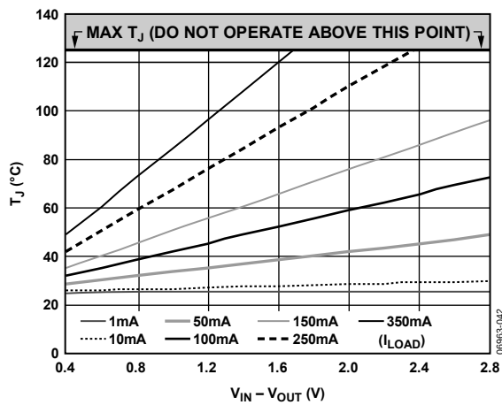
Figure 42. 0 \text{mm}^2 of PCB Copper, T_A = 25^{\circ}\text{C} , TSOT
