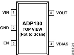
Figure 3. Pin Configuration
