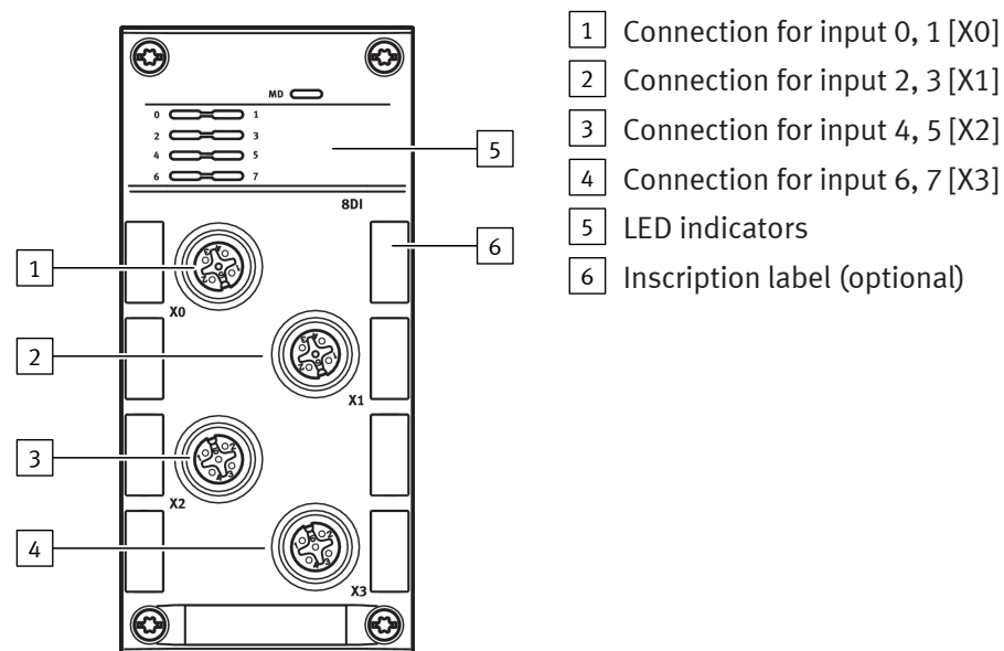
Fig. 1: Product design
