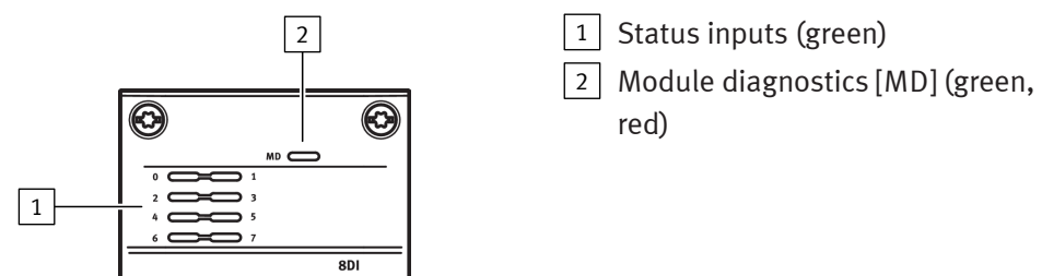
Fig. 2: LED indicators
