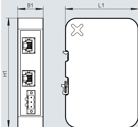
Dimensions – Power supply unit CACN
