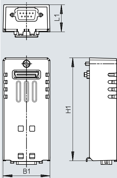
Dimensions – Bus interface CDPX-F-CO
