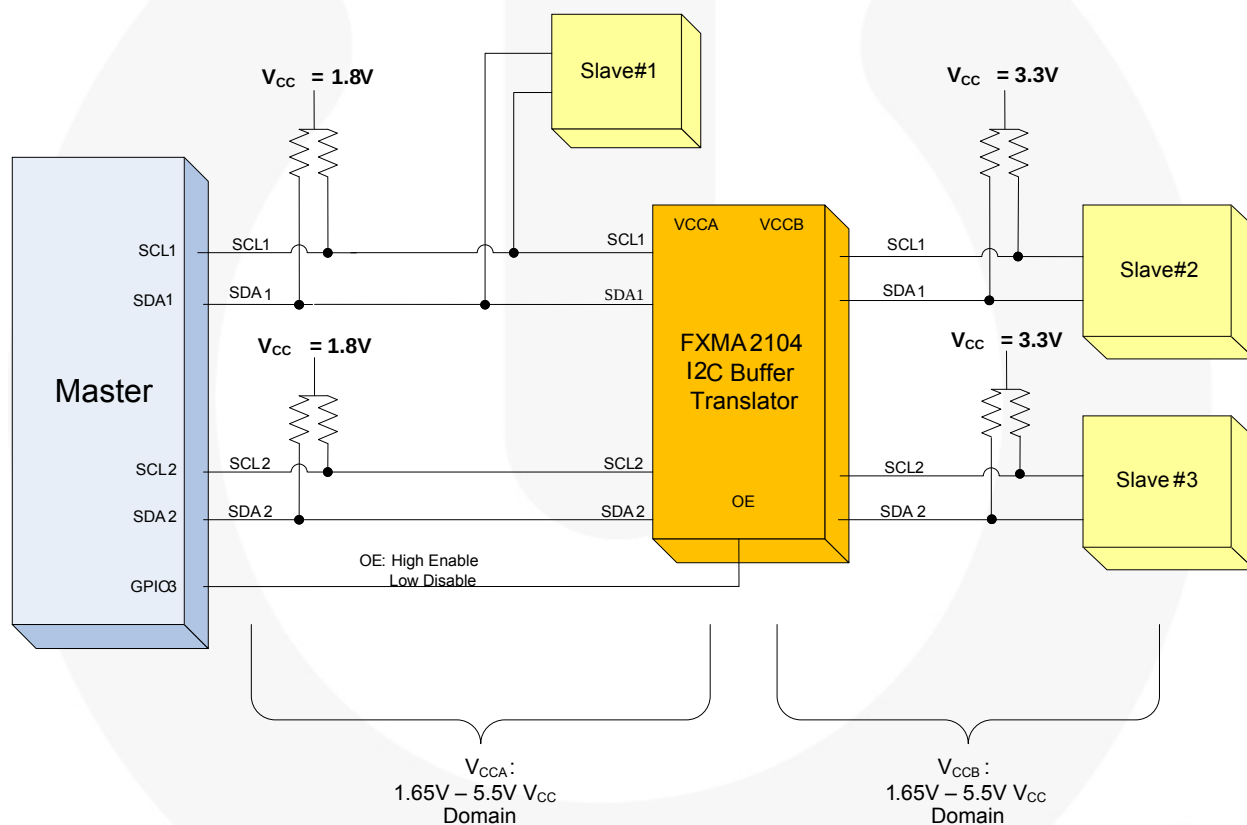
Figure 6. Bus Isolation
