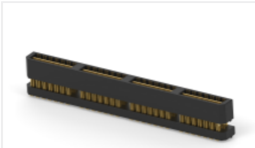
TE Part # 1658438-4 MSB0.80PL14ASY160FL,-,10,-TY
