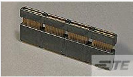
TE Part # 1658051-4 MSB0.80PL30ASY160FL,-,F,-TY
