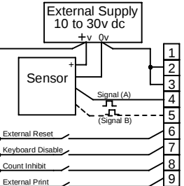
Illustrating use of external power supply (source mode depicted).
