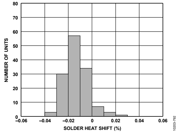
Figure 82. ADR4550 Solder Heat Resistance Shift (3 × Reflow)
