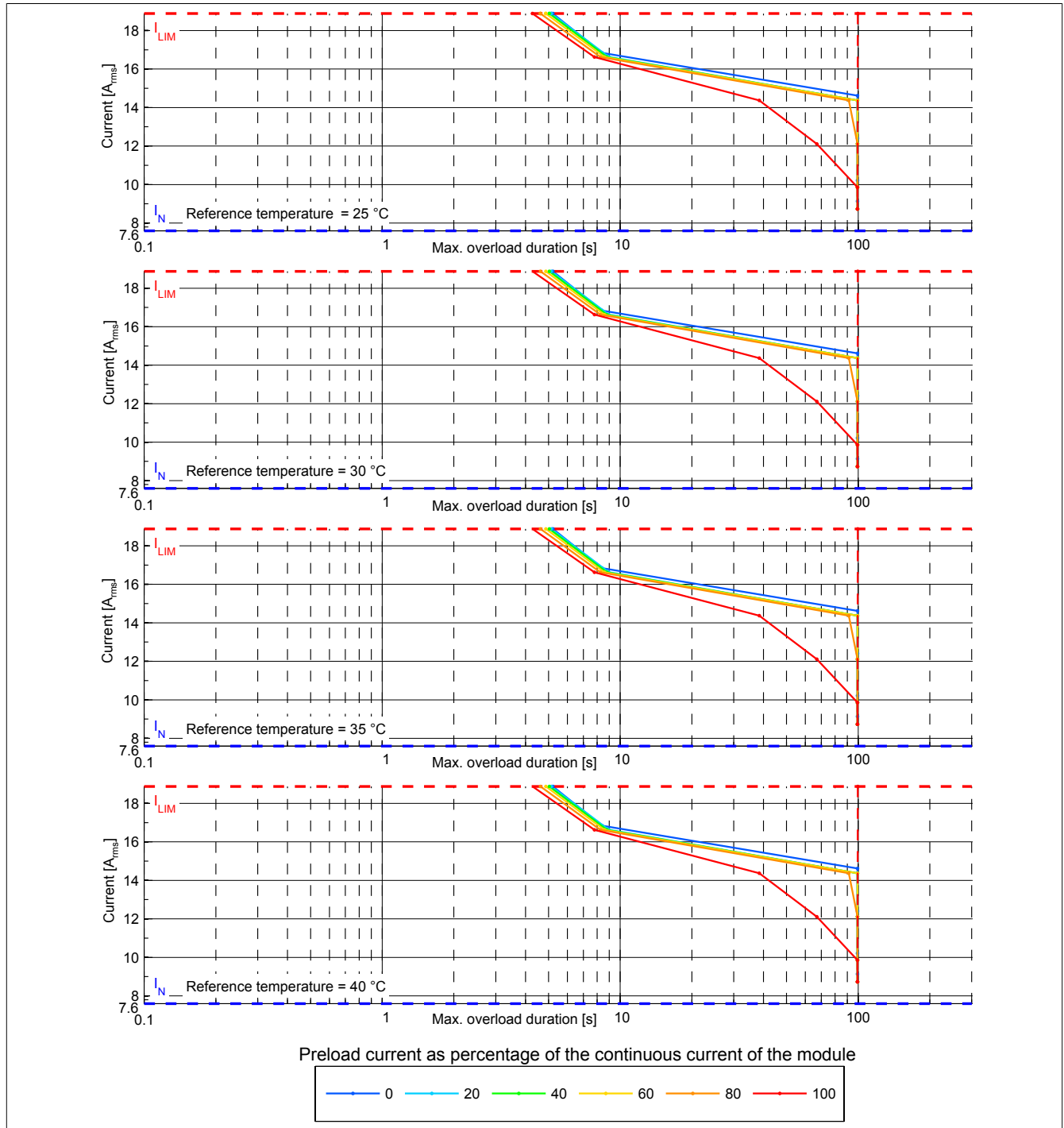
Figure 1: 8BVI0055HWDx.000-x - Overload characteristics, overload response - WARNING
