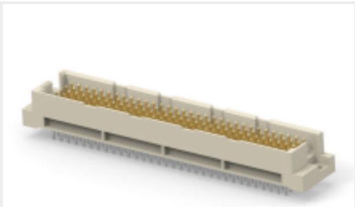
TE Part #374472-E STVTE 160 MI ABCDE VVVV 4-00 GA06 4,0 *
