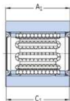
LUJR With shaft seals
