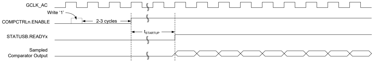
Figure 37-3. Continuous Measurement Example
