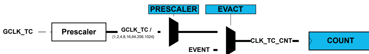
Figure 33-2. Prescaler
