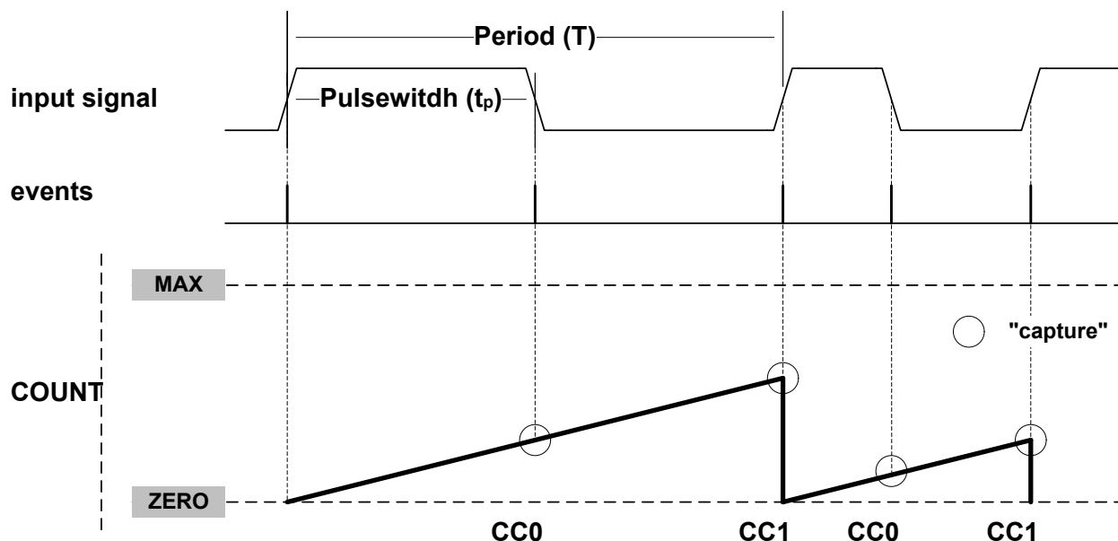
Figure 33-13. PWP Capture
