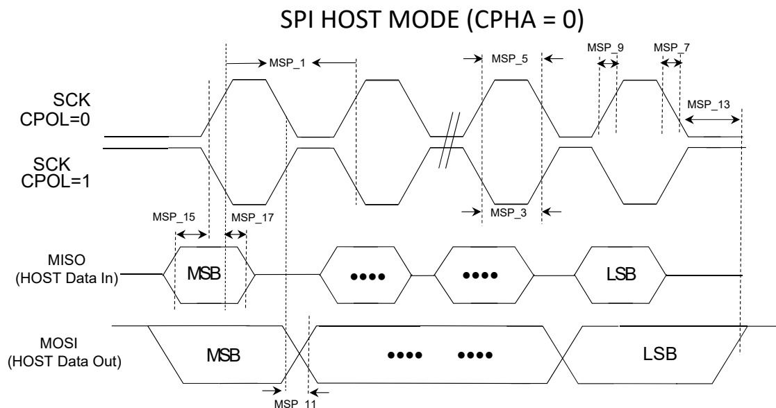
Figure 40-1. SPIx Host Module CPHA = 0 Timing Diagrams
