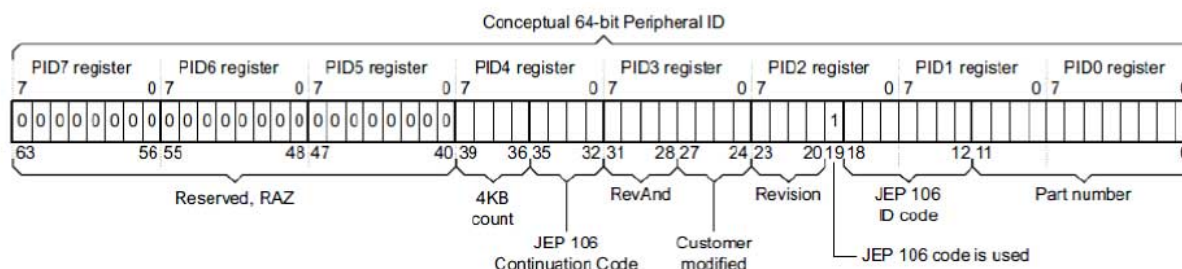
Figure 20-5. Conceptual 64-bit Peripheral ID
