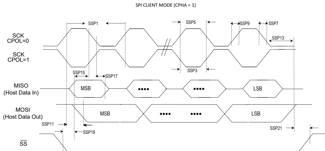
Figure 39-7. SPIx Client Module (CPHA = 1) Timing Diagrams
