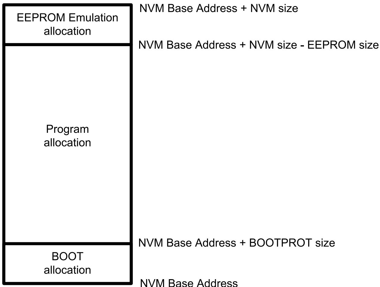
Figure 26-4. EEPROM and Boot Loader Memory Allocation
