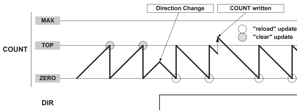
Figure 34-3. Counter Operation
