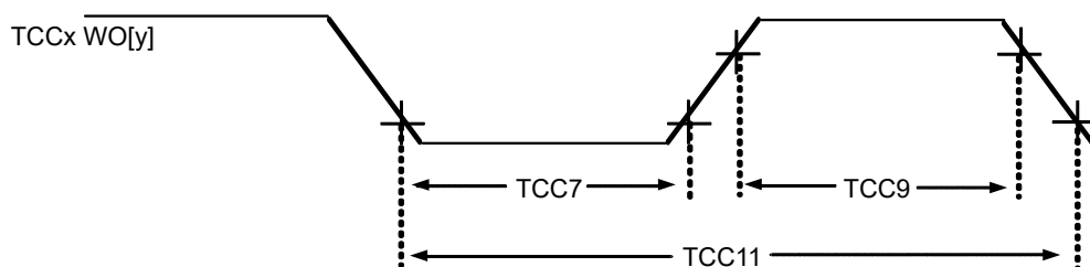
Figure 39-15. TCC0/1 Timer Compare Output Timing Diagrams
