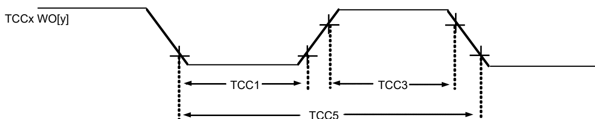
Figure 39-15. TCC0/1 Timer Compare Output Timing Diagrams
