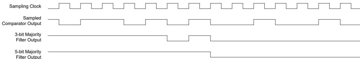
Figure 37-8. Single-Shot Filtering
