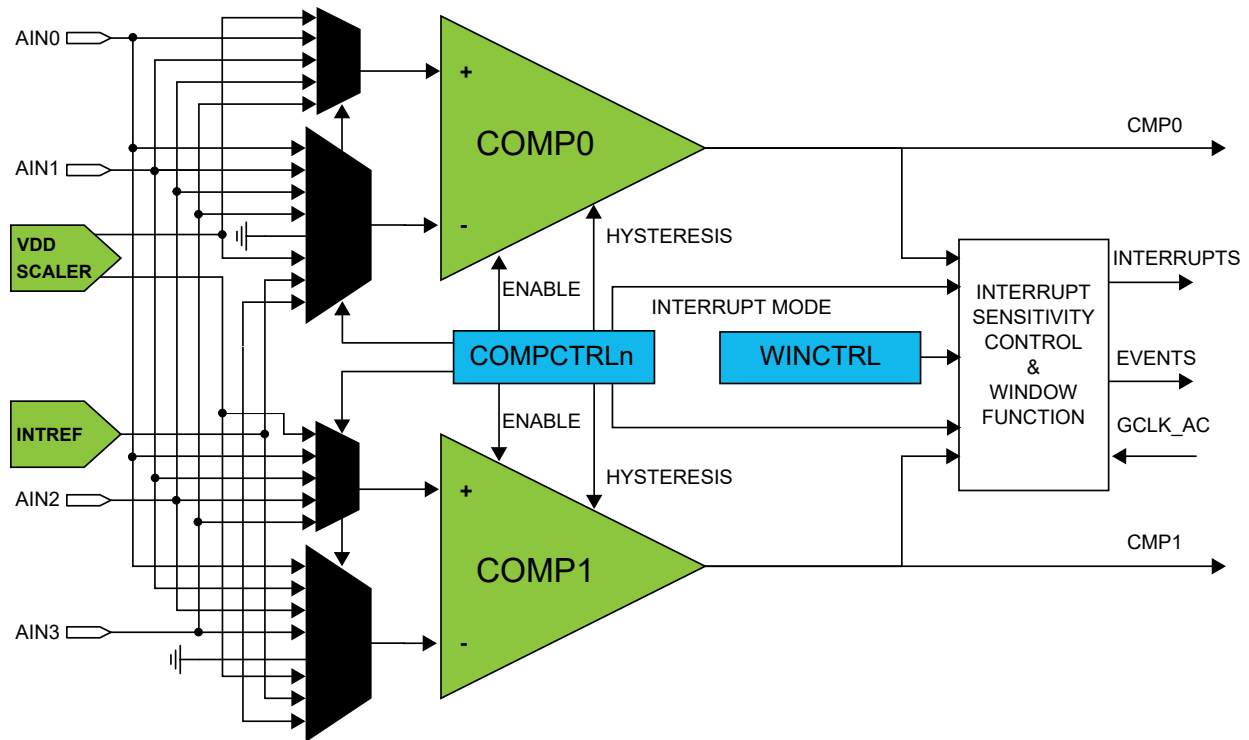
Figure 37-1. Analog Comparator Block Diagram (First Pair)
