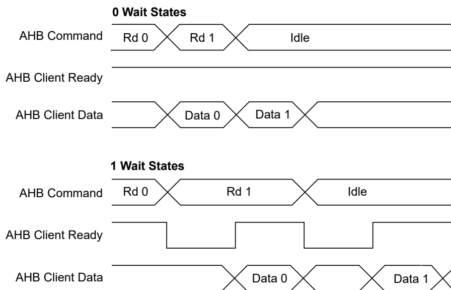
Figure 26-5. Read Wait State Examples
