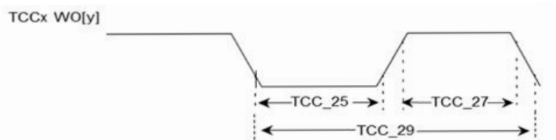
Figure 39-17. TCC2 Timer Compare Output Timing Diagrams
