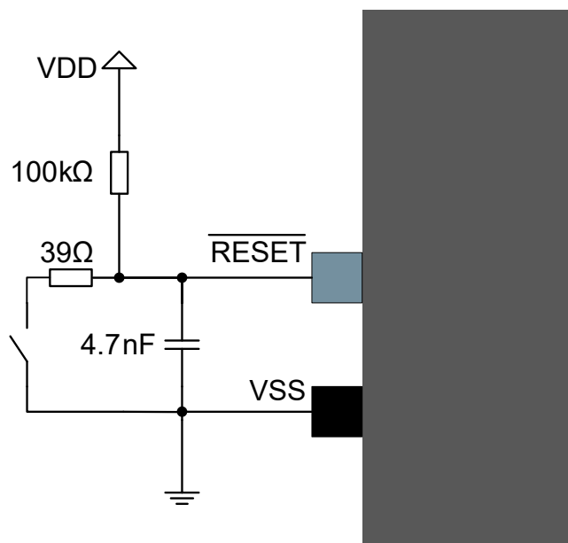
Figure 42-4. External Reset Circuit Schematic (General Purpose) (2)
