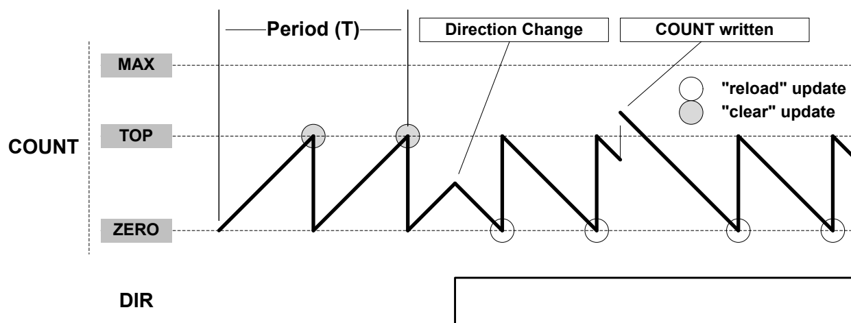
Figure 33-3. Counter Operation
