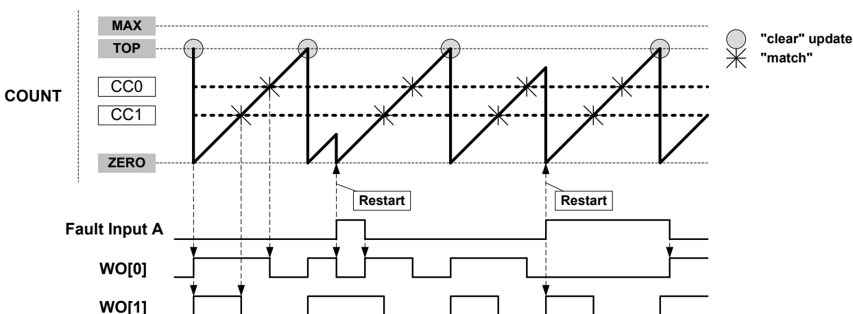
Figure 34-26. Waveform Generation in RAMP1 mode with Restart Action
