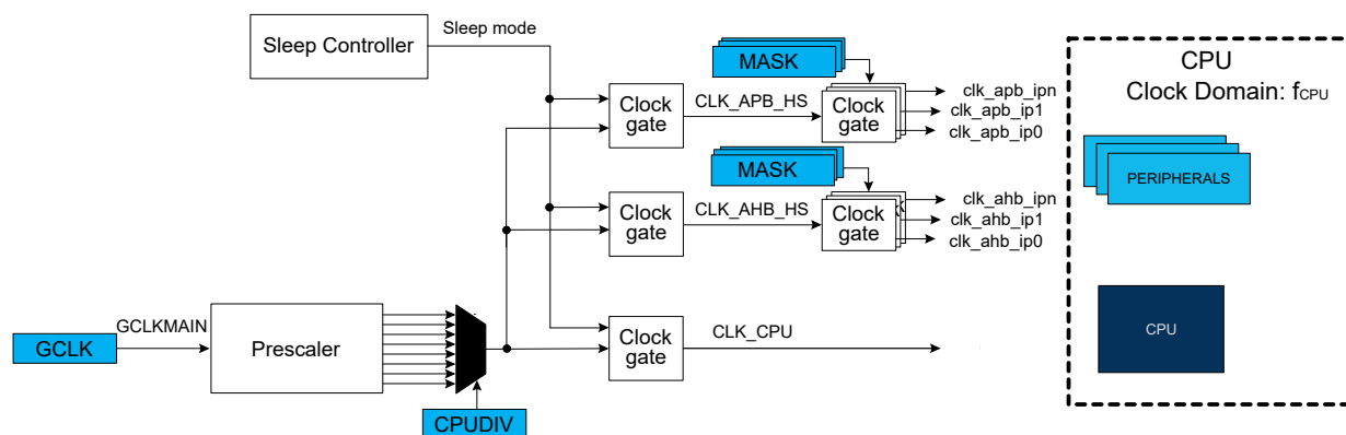
Figure 13-2. Synchronous Clock Selection and Prescaler
