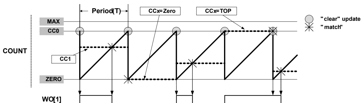
Figure 33-6. Match PWM Operation
