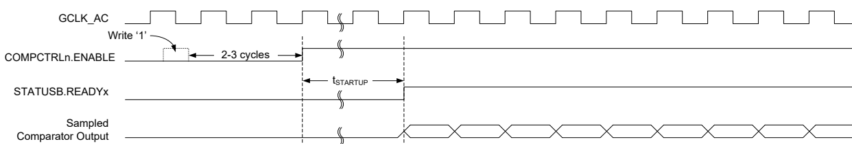
Figure 37-10. Continuous Mode SleepWalking
