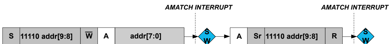
Figure 32-12. 10-bit Addressing
