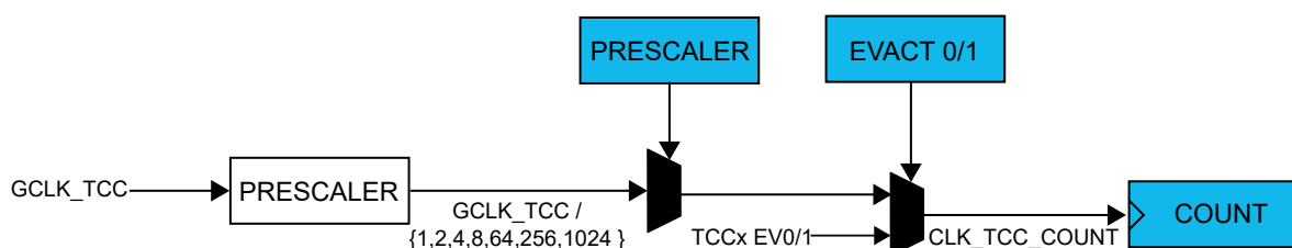
Figure 34-2. Prescaler
