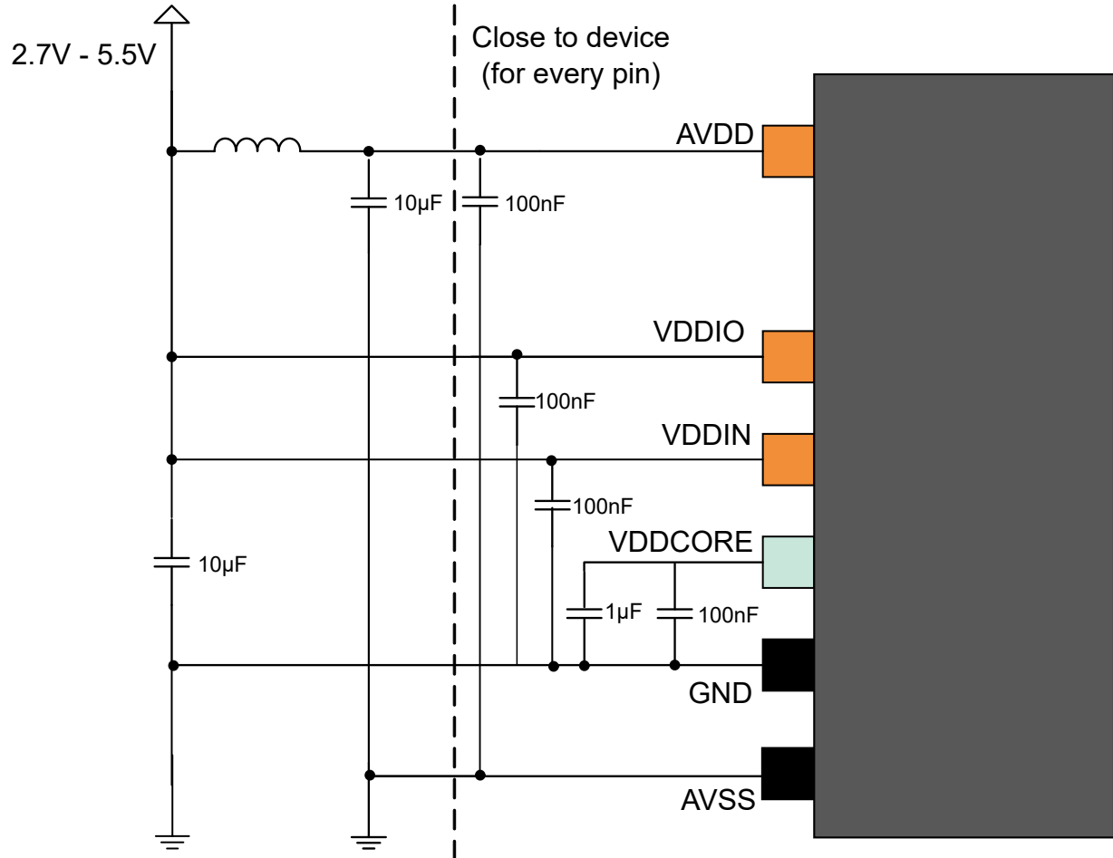
Figure 42-1. Single Power Supply Schematic
