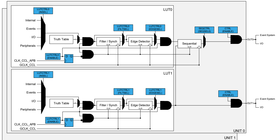
Figure 35-1. Configurable Custom Logic
