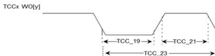
Figure 39-16. TCC2 Timer Capture Input Timing Diagram
