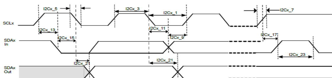
Figure 39-11. I 2 C Bus Data Client Mode AC Timing Diagrams
