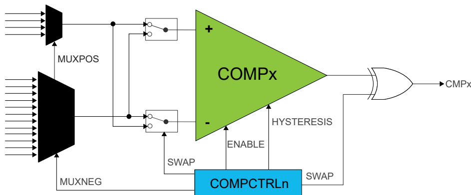
Figure 37-9. Input Swapping for Offset Compensation
