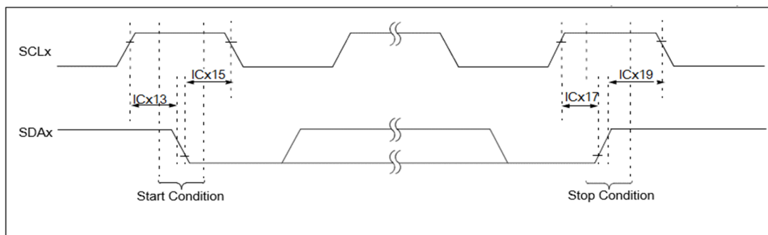
Figure 39-9. I 2 C Bus Data Host Mode AC Timing Diagrams
