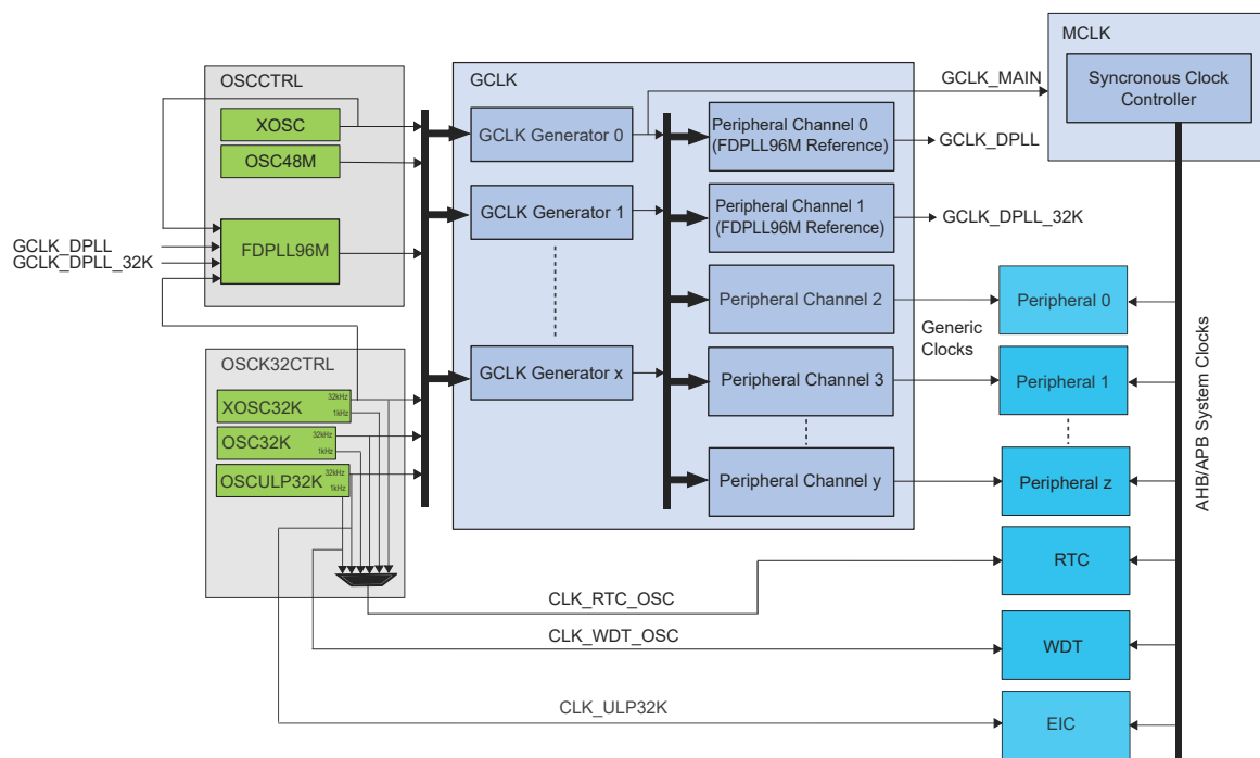
Figure 11-1. Clock distribution
