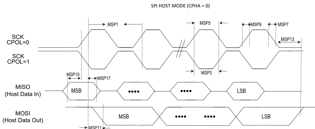
Figure 39-4. SPIx Host Module (CPHA = 0) Timing Diagrams
