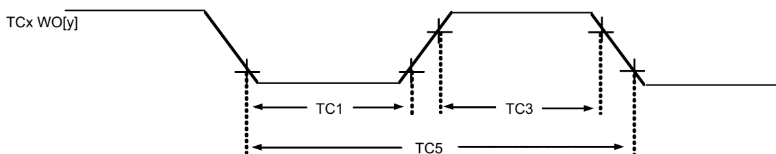
Figure 39-13. TCx Timer Compare Output Timing Diagrams
