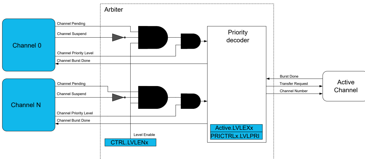
Figure 24-4. Arbiter Overview
