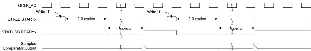
Figure 37-4. Single-Shot Example
