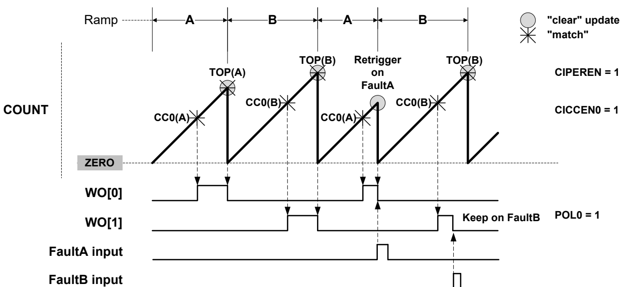
Figure 34-19. RAMP2 Alternate Operation
