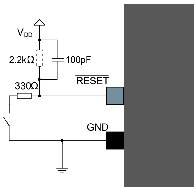
Figure 42-5. External Reset Circuit Schematic (EFT Immunity Enhancement) (2)
