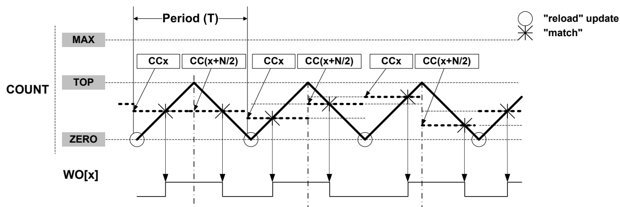
Figure 34-8. Dual-Slope Critical Pulse Width Modulation ( N=\text{CC\_NUM} )
