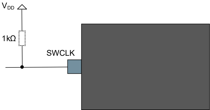
Figure 42-9. SWCLK Circuit Connections
