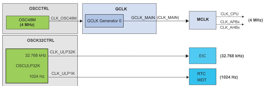
Figure 6-2. Clocks Distribution after Reset (Simplified)
