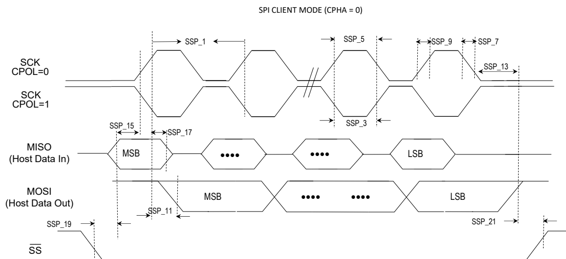
Figure 40-3. SPIx Client Module CPHA = 0 Timing Diagram
