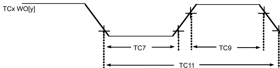
Figure 39-13. TCx Timer Compare Output Timing Diagrams
