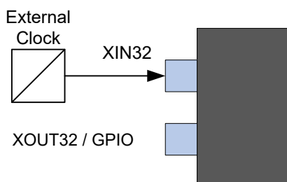
Figure 42-8. 32.768 kHz External Clock Source Schematic
