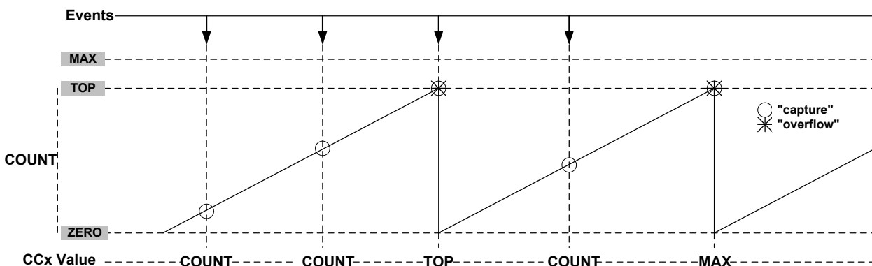
Figure 33-15. Time-Stamp
