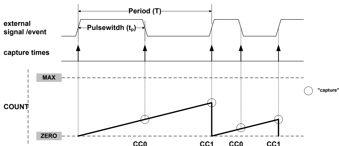
Figure 34-16. PWP Capture
