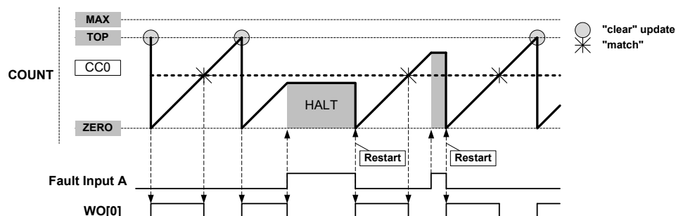
Figure 34-31. Waveform Generation with Fault Qualification, Halt, and Restart Actions
