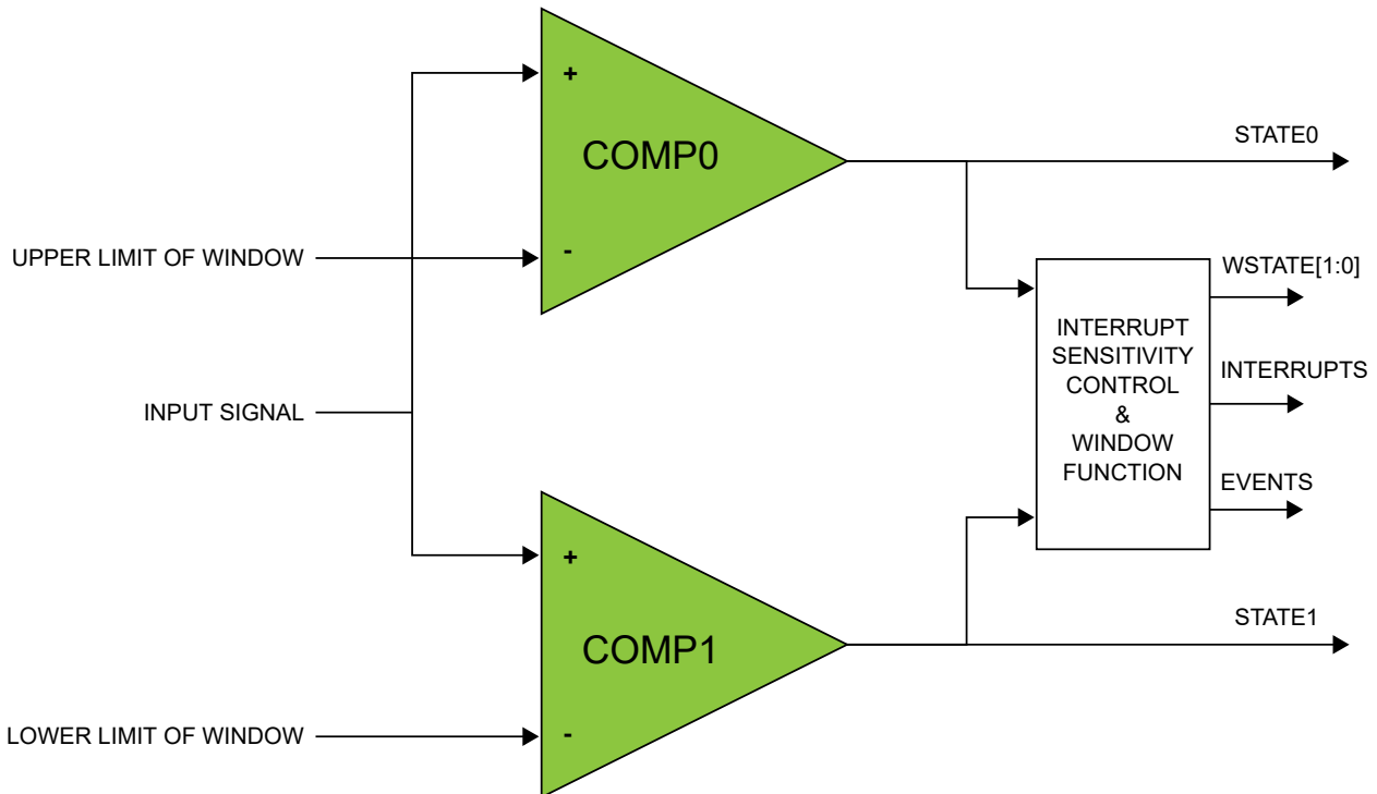
Figure 37-5. Comparators in Window Mode
