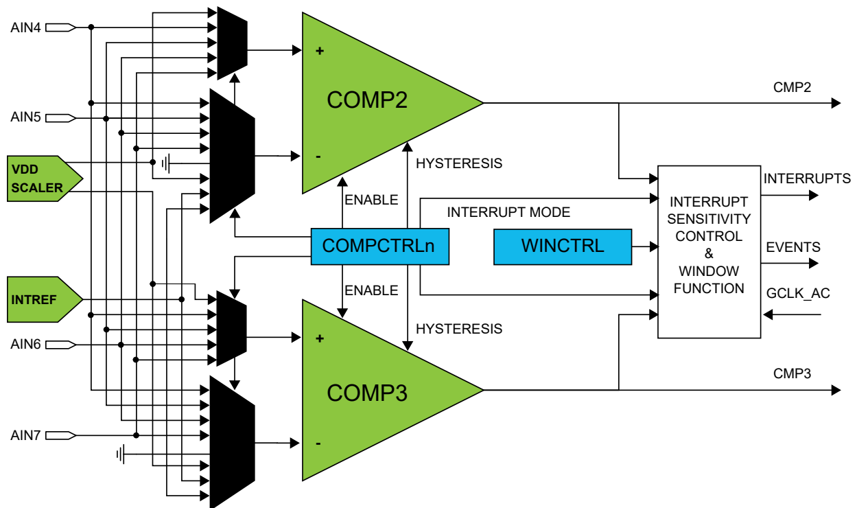
Figure 37-2. Analog Comparator Block Diagram (Second Pair)
