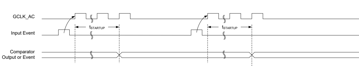
Figure 37-11. Single-Shot SleepWalking
