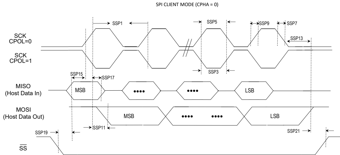
Figure 39-6. SPIx Client Module (CPHA = 0) Timing Diagrams
