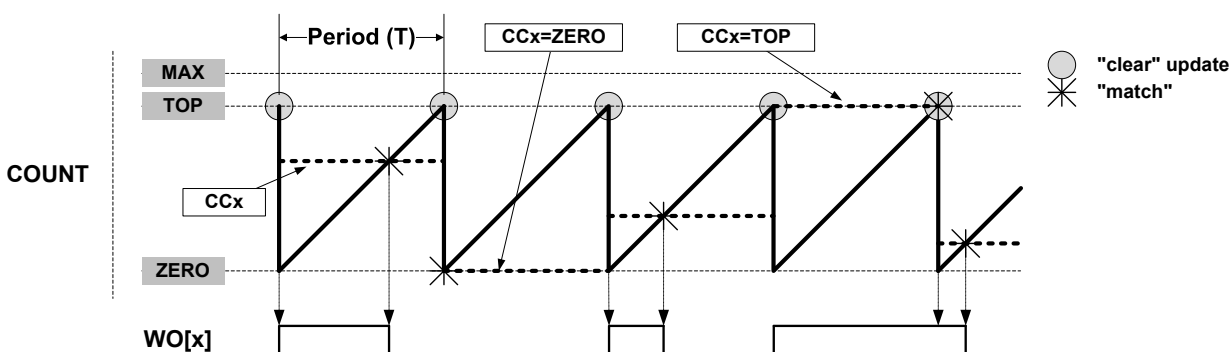
Figure 34-6. Single-Slope PWM Operation
