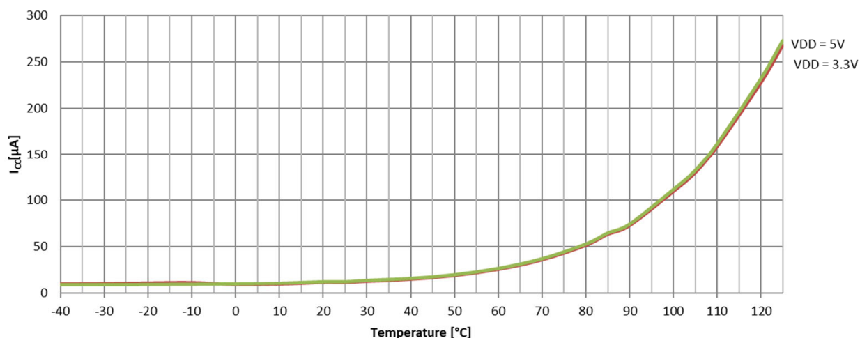
Figure 39-1. Standby Power Consumption over Temperature with Typical Material
