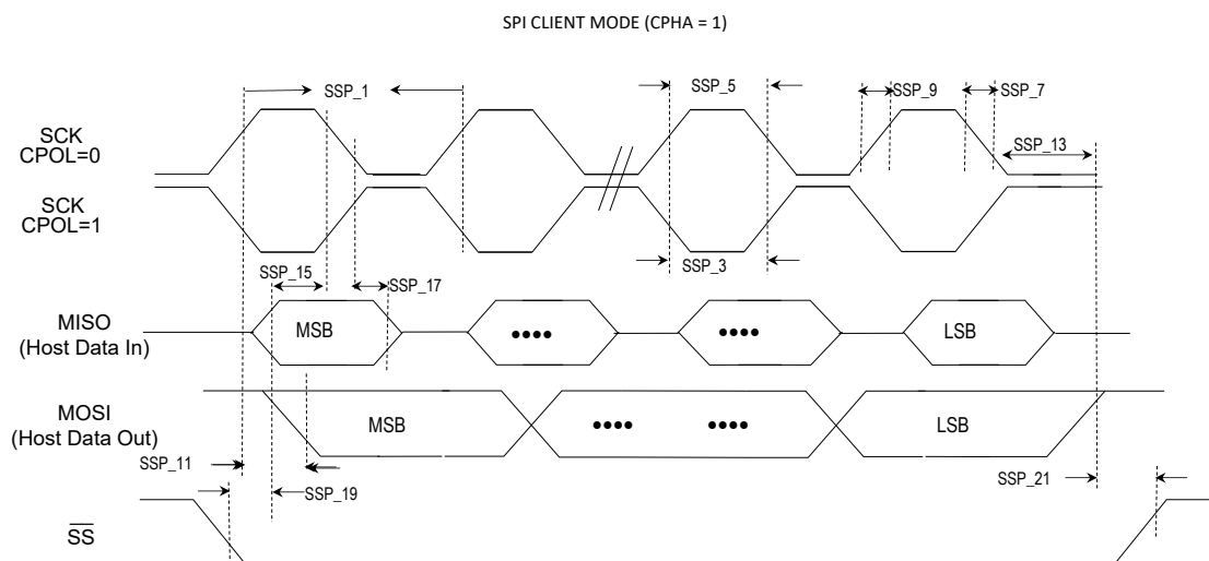
Figure 40-4. SPIx Client Module CPHA = 1 Timing Diagram
