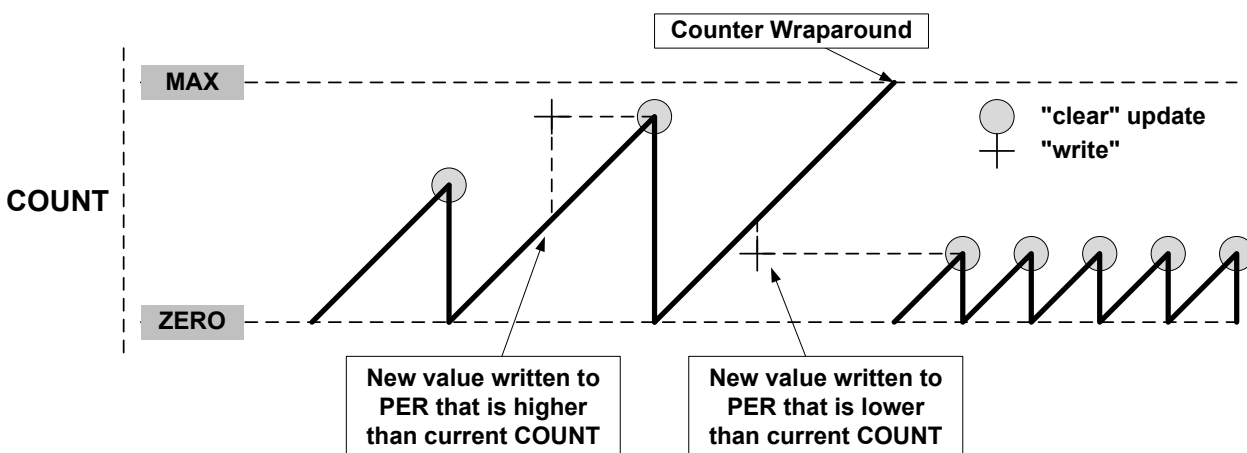
Figure 34-10. Unbuffered Single-Slope Up-Counting Operation
