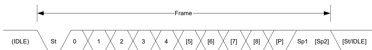
Figure 30-2. Frame Formats
