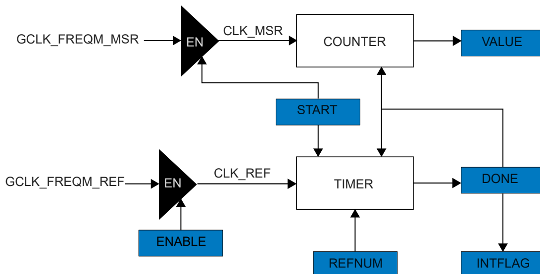
Figure 38-1. FREQM Block Diagram
