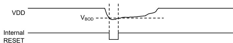
Figure 17-2. BOD Hysteresis Principle
