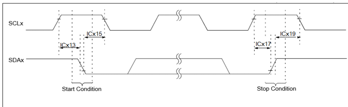
Figure 39-11. I 2 C Bus Data Client Mode AC Timing Diagrams
