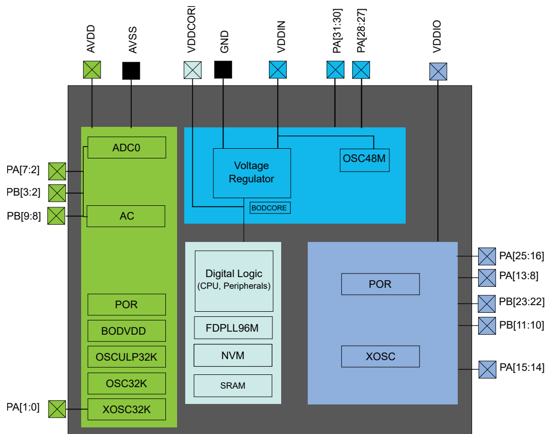
Figure 6-1. Power Domain Overview - PIC32CM JH00
