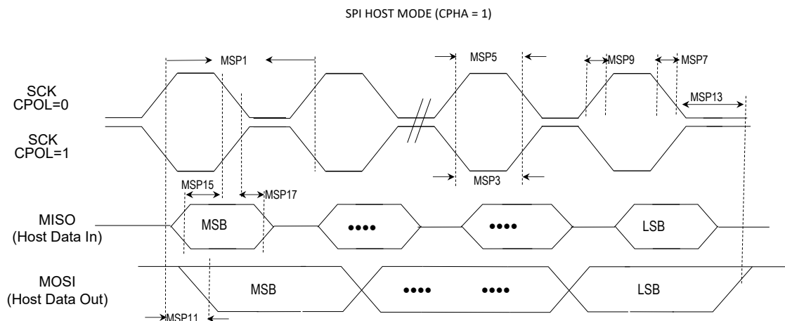
Figure 39-5. SPIx Host Module (CPHA = 1) Timing Diagrams
