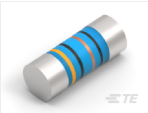
TE Part #7-2176315-1 MELF SMA_A 56K 1% 50PPM 0204 0.4 W
