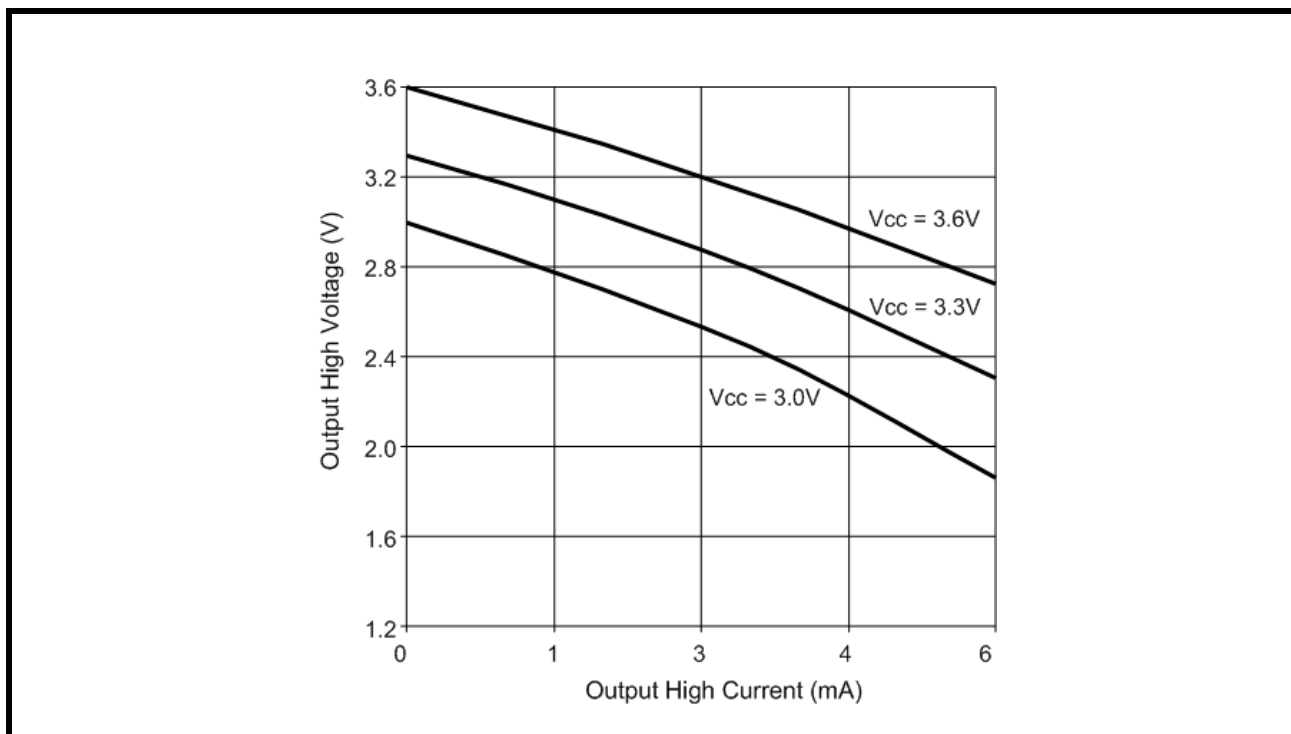
FIGURE 21. V OUT HIGH VS I OUT (V CC )
