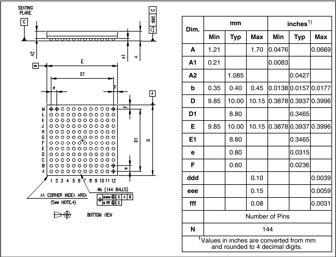
Figure 29. 144-Low Profile Fine Pitch Ball Grid Array Package
