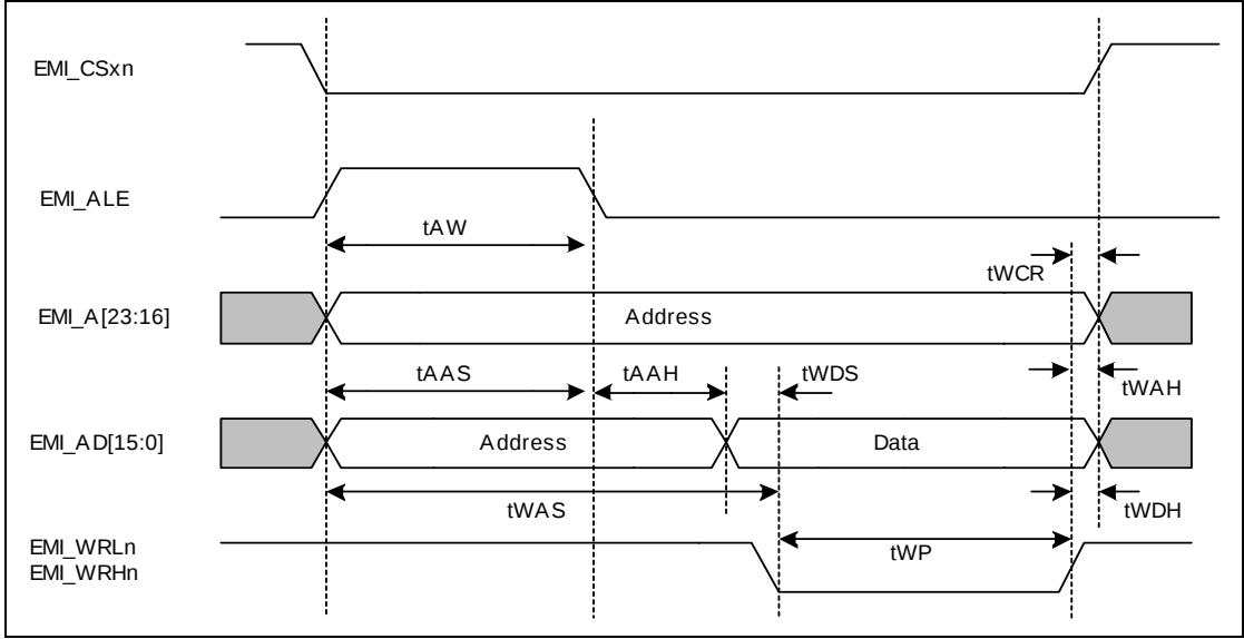
Figure 16. Mux Bus (16-bit) Write Timings
