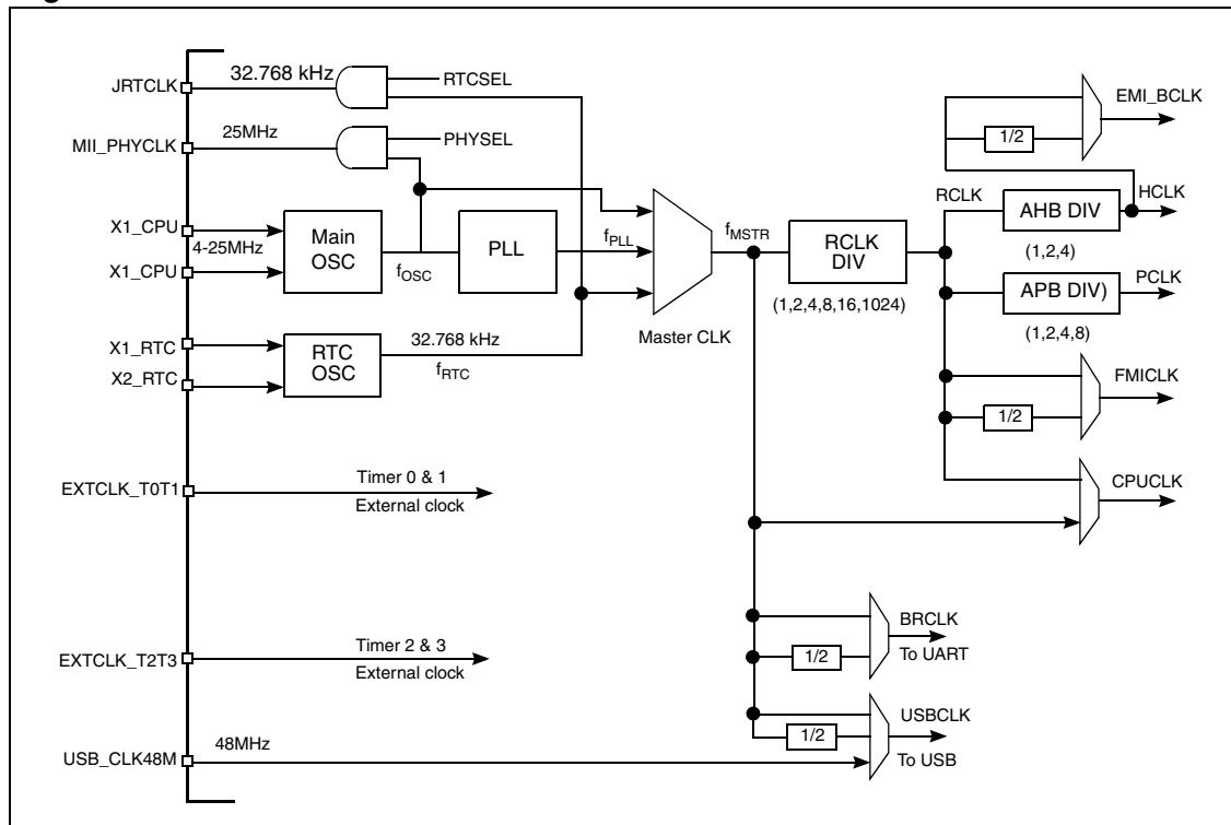
Figure 2. Clock control
