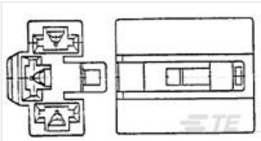
TE Part #176774-5 FF 250 PLUG HSG 3P NYLON NAT
