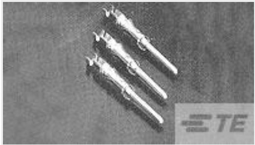
TE Part # 1-1108757-1 HSK.Sti.C.1,5 qmm
