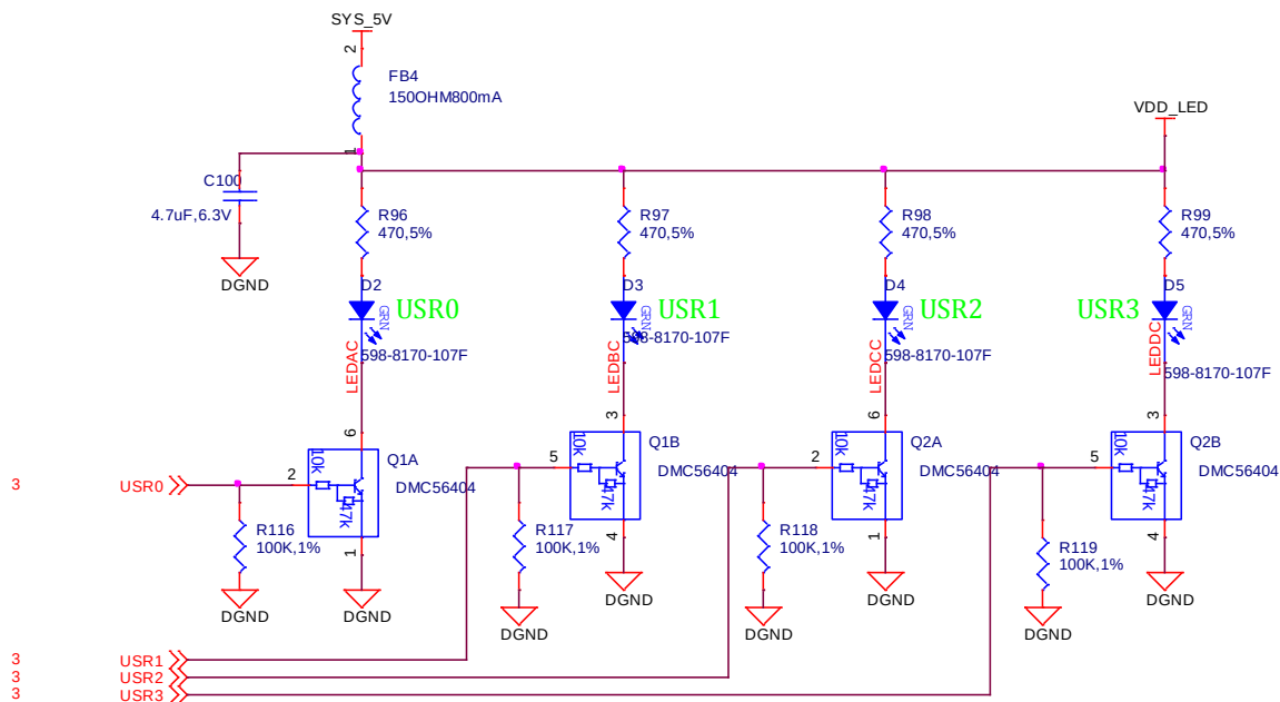
Figure 19. User LEDs
