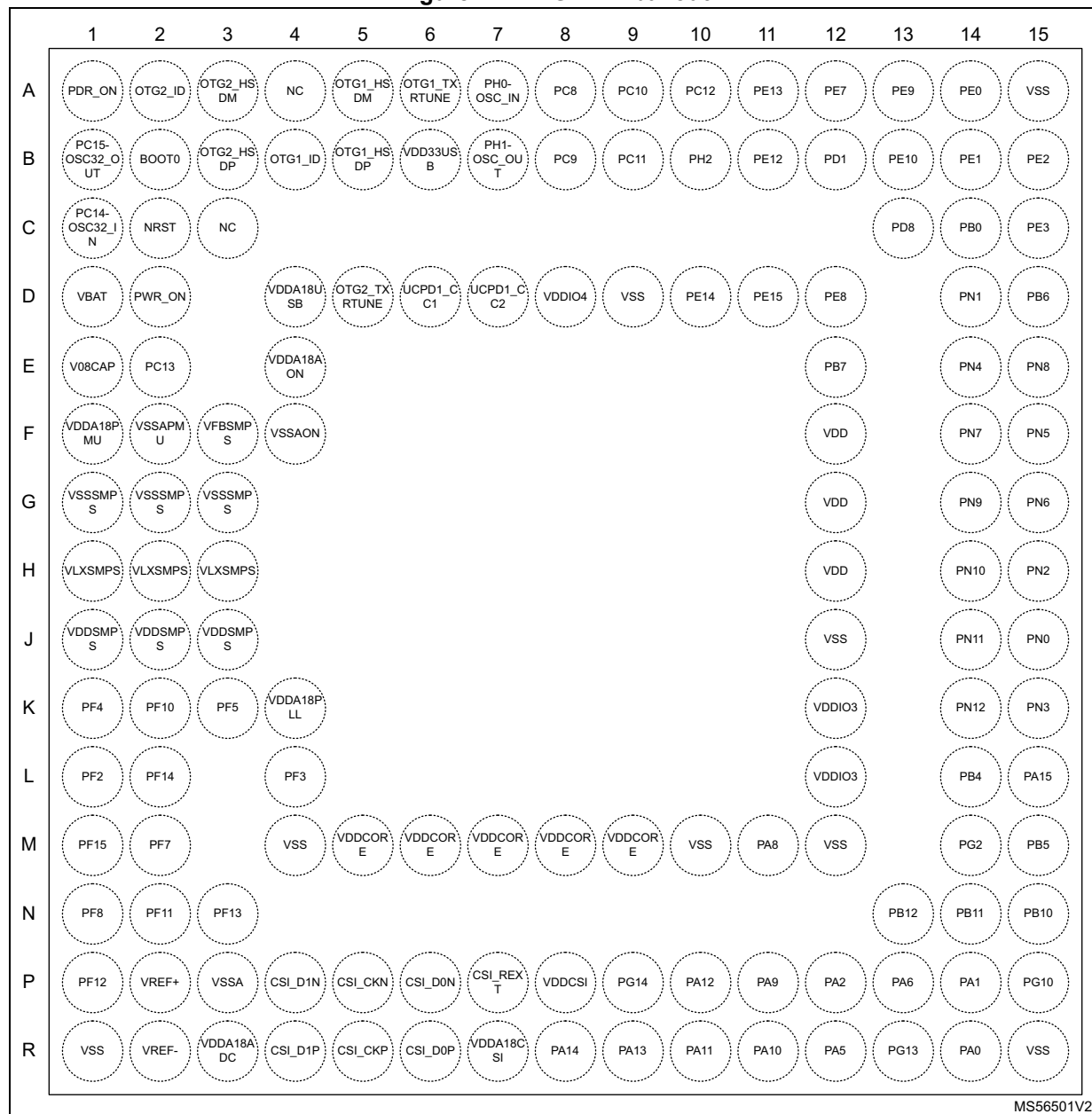
Figure 7. VFBGA142 ballout
