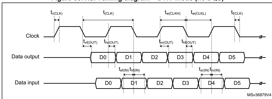
Figure 35. XSPI timing diagram – DTR mode (no DQS)
