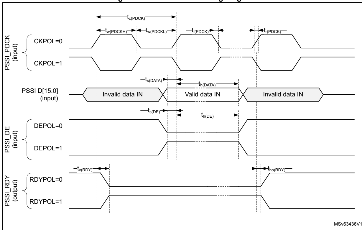
Figure 50. PSSI receive timing diagram
