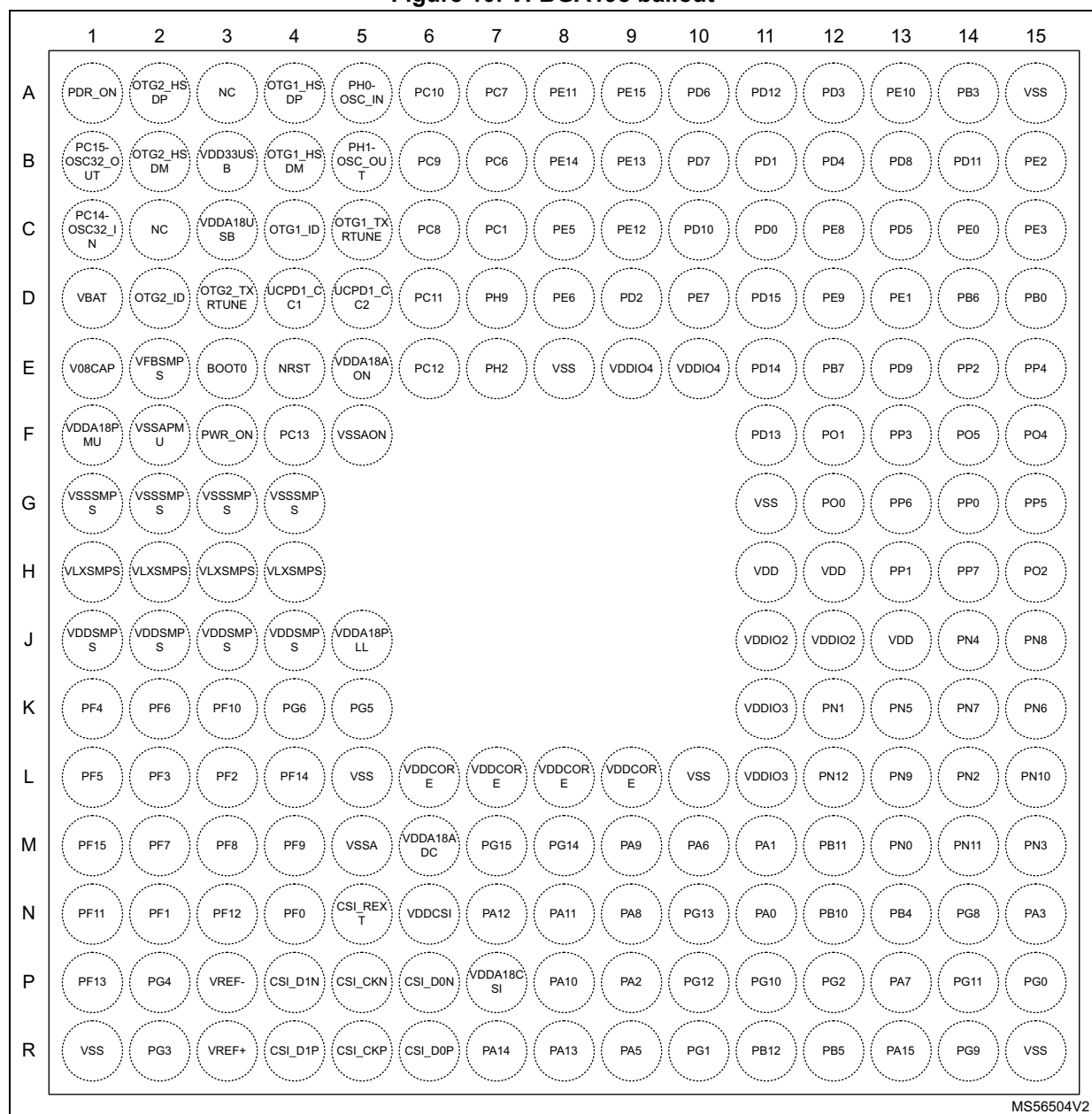
Figure 10. VFBGA198 ballout
