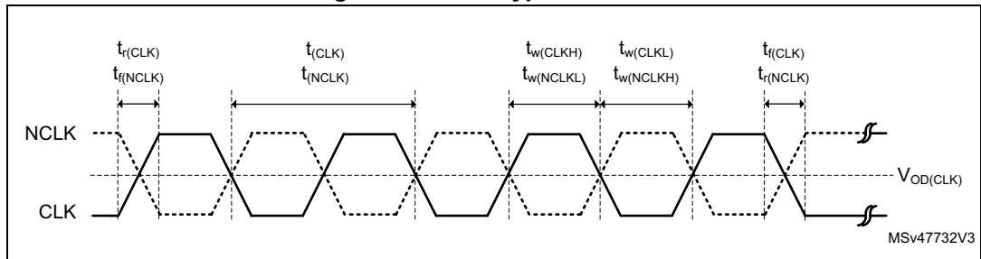
Figure 36. XSPI HyperBus clock
