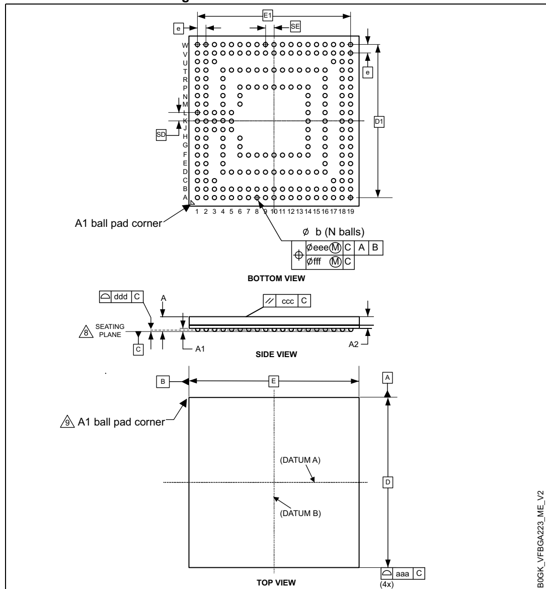
Figure 70. VFBGA223 - Outline (13)
