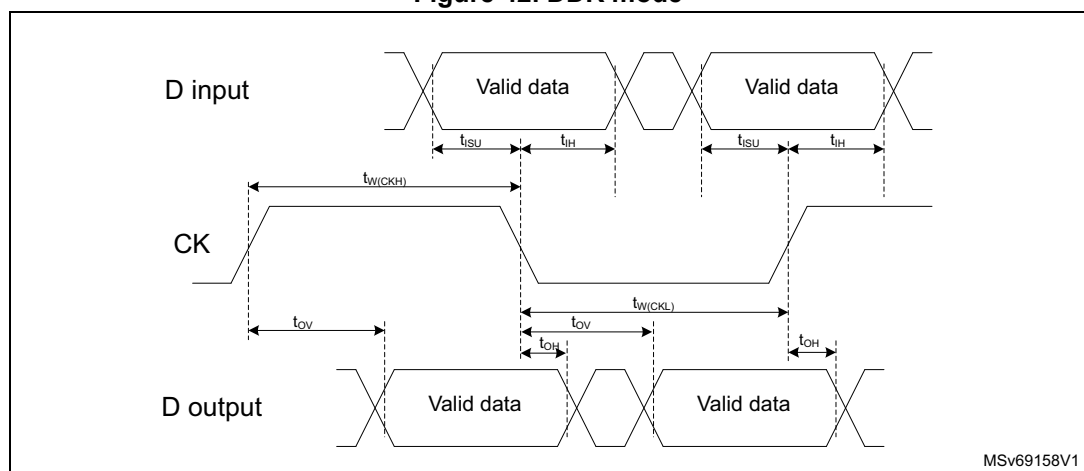
Figure 42. DDR mode
