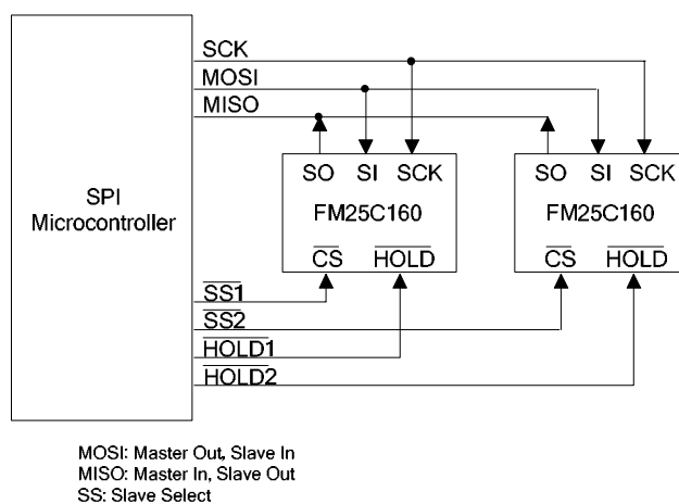
Figure 2. System Configuration with SPI port
