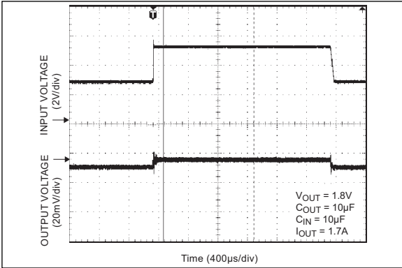
FIGURE 2-11: Line Transient.
