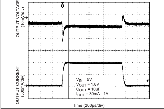
FIGURE 2-12: Load Transient.
