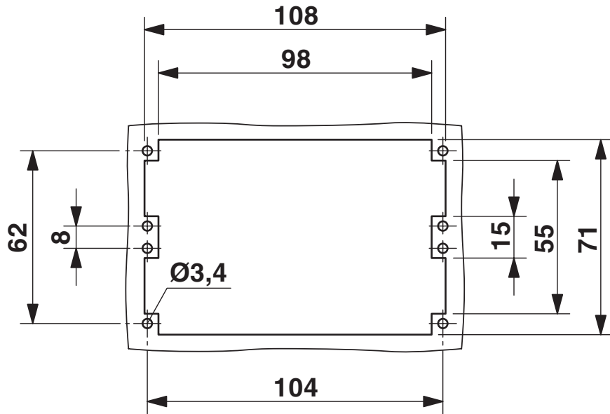
Dimensional drawing
