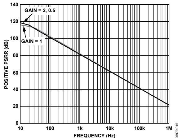
Figure 13. Positive PSRR vs. Frequency
