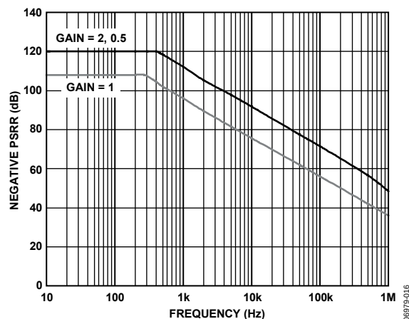
Figure 14. Negative PSRR vs. Frequency
