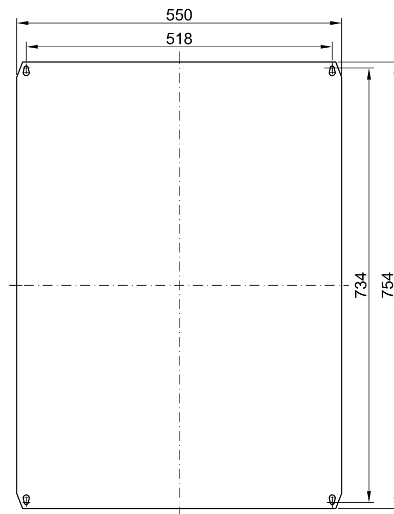
Base Plate
