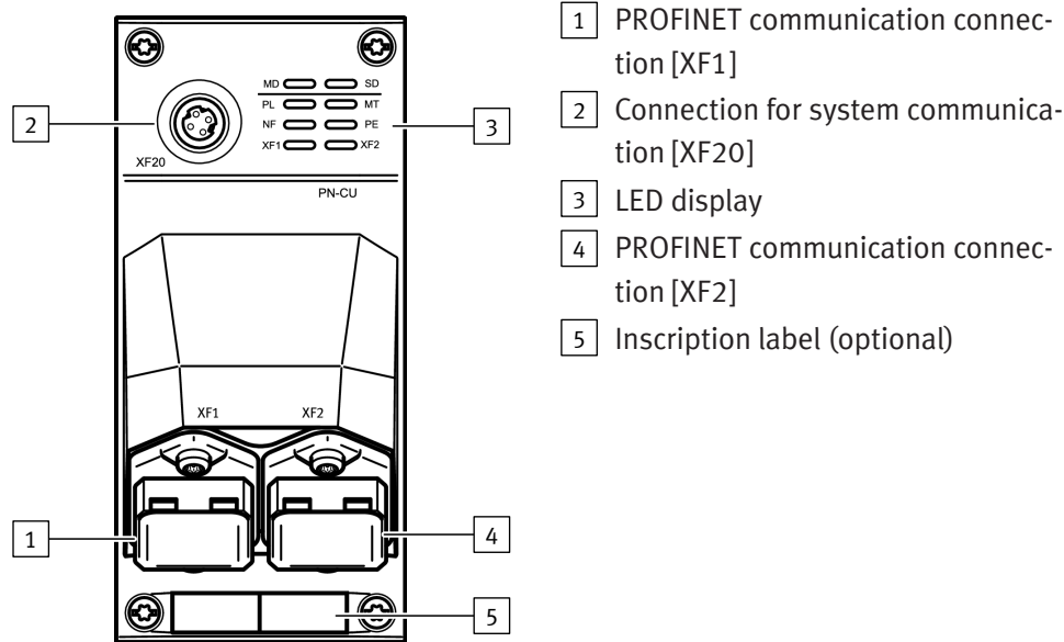
Fig. 1: Product design
