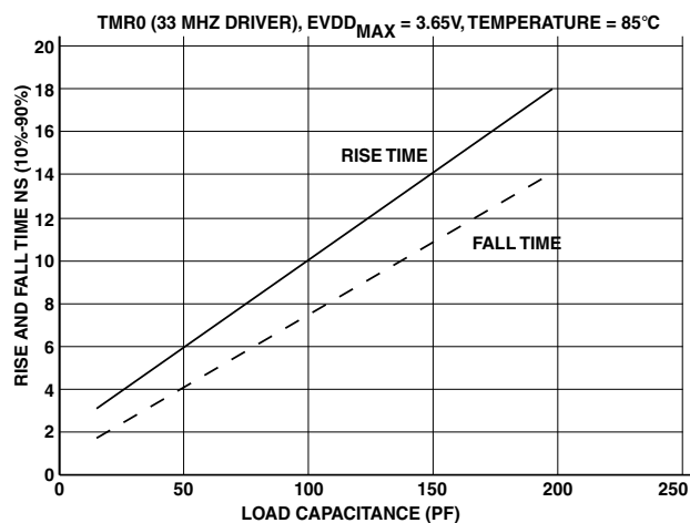
Figure 41. Typical Output Delay or Hold for Driver C at EVDD_{MAX}
