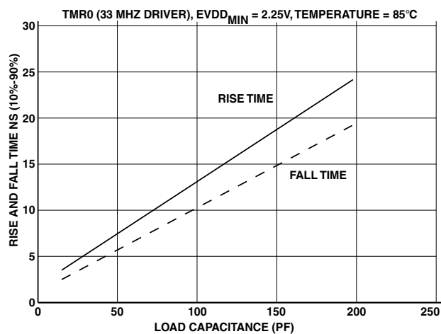
Figure 40. Typical Output Delay or Hold for Driver C at EVDD_{MIN}
