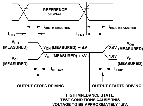
Figure 33. Output Enable/Disable
