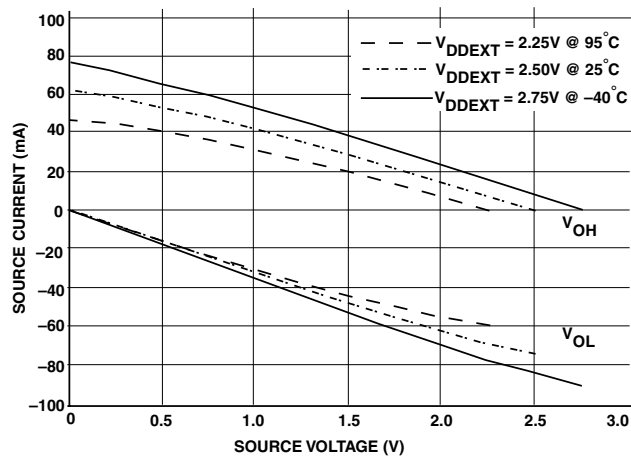
Figure 31. Drive Current D (Low V_{DDEXT} )
