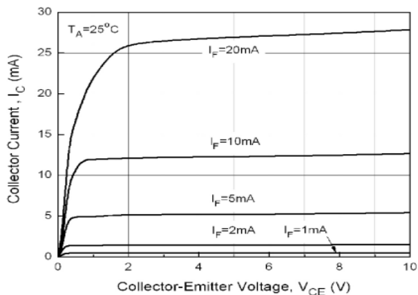
Fig 5 Collector Current vs Collector-Emmitter Voltage (1)
