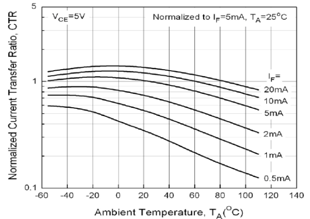
Fig 8 Normalized CTR vs Ambient Temperature
