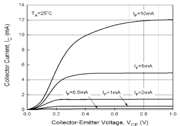
Fig 6 Collector Current vs Collector-Emmitter Voltage (2)
