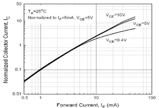
Fig 4 Normalized Collector Current vs Forward Current
