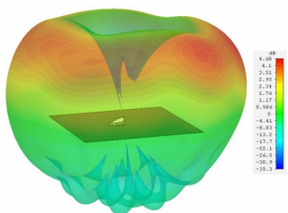
4G-element 1800 MHz, side view
