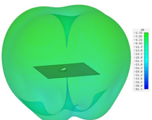
UHF-element 380 MHz, side view
