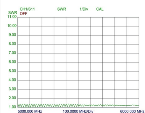
TYPICAL VSWR CURVE WIFI 5.6 GHz *
