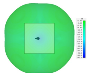
UHF-element 380 MHz, top view
