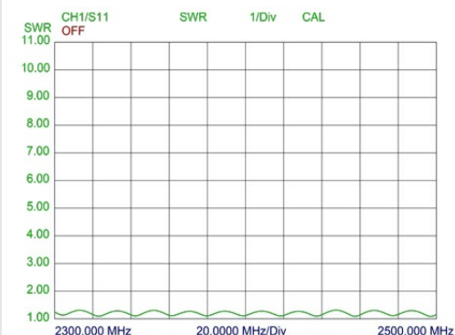
TYPICAL VSWR CURVE INBUILT-UHF WITH WHIP **
