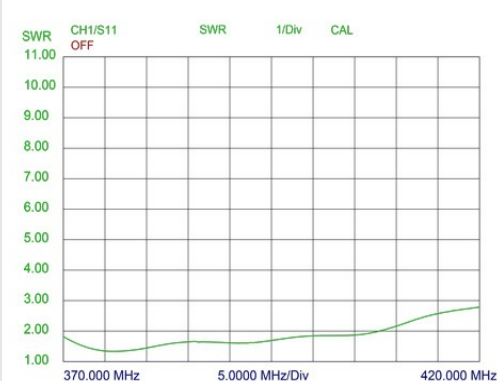
TYPICAL VSWR CURVE INBUILT-UHF WITH WHIP **
