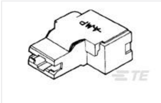
TE Part #1-172469-2 PL 250 (6.3 MM) HOUSING BLUE 6/6 NYLON
