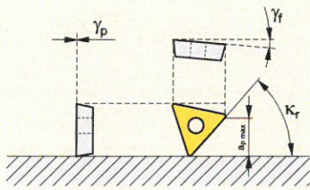
Abmessungen [mm]. / Dimensions [mm].
