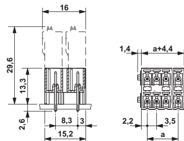
Dimensioned drawing
