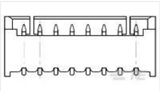
TE Part #1734829-4 1.25 WTB HDR DIP, 4 POS
