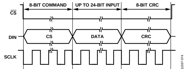
Figure 50. SPI Write Transaction with CRC
