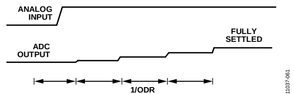
Figure 37. Step Input Without Single Cycle Settling
