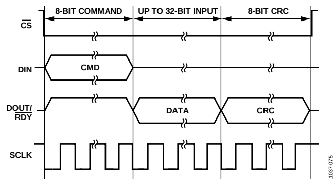
Figure 51. SPI Read Transaction with CRC
