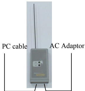
Figure 9: the Receiver
