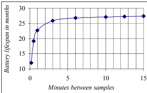
Figure 2: MicroLog battery life
