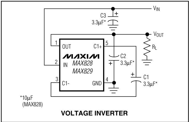
Figure 1. Test Circuit
