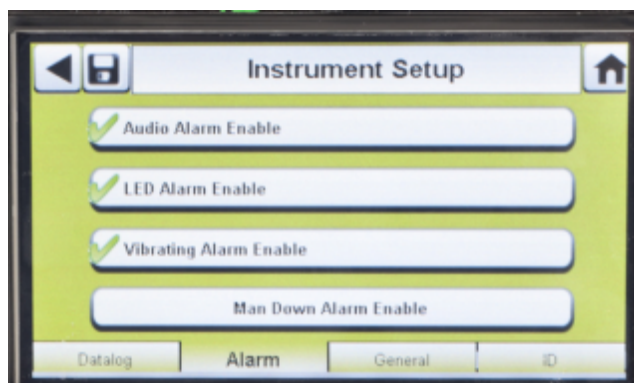
Figure 18 Instrument Setup - Alarm
