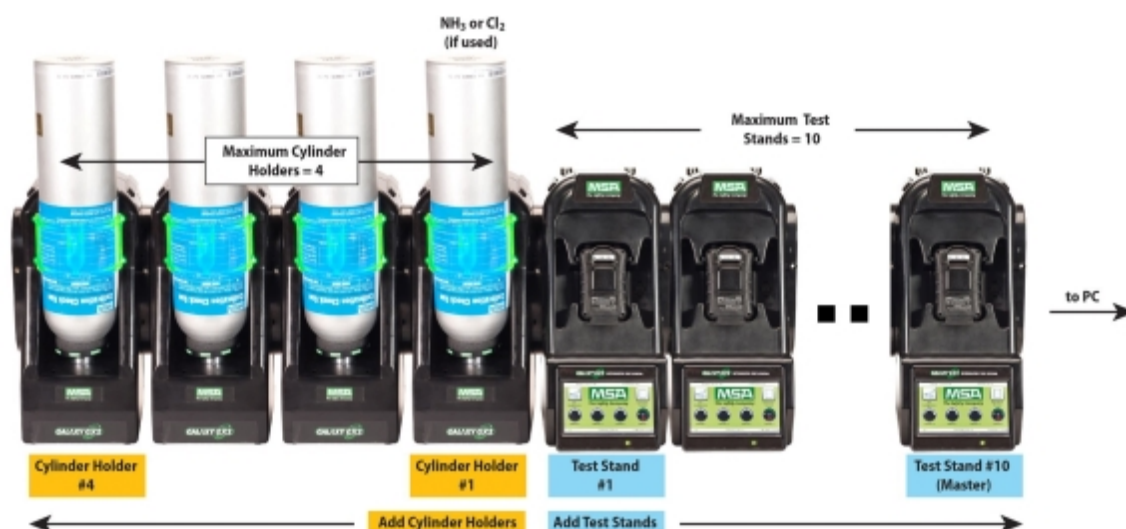
Figure 8 Test Stands and Cylinder Holders properly installed in a bank
