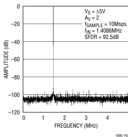
Figure 3. 4096 Point FFT Response
