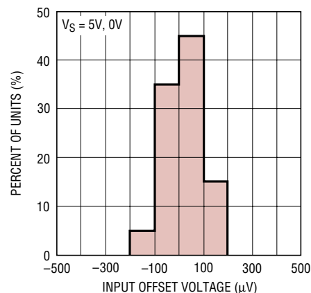
\Delta V_{OS} Shift for V_{CM} = 0\text{V} to 5\text{V}
