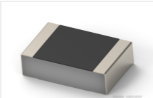
TE Part #3-2176453-3 CPF 0201 12K4 0.1% 25ppm 1K RL
