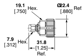
Part No. 1053646-1
