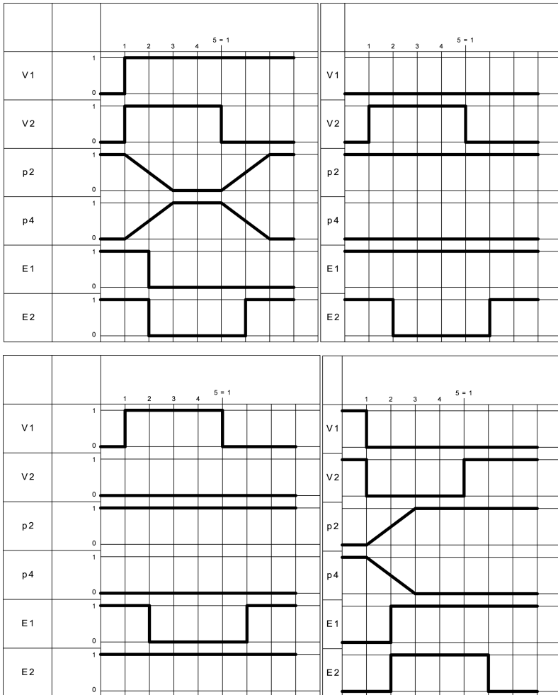
Fig. 10: Function test, steps 3 to 6
