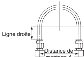
Fig. 1 Raccordement recommandé
