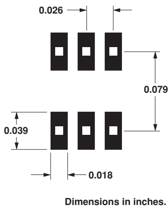
Figure 20. Recommended PCB Pad Layout for Avago's SC70 6L/SOT-363 Products.
