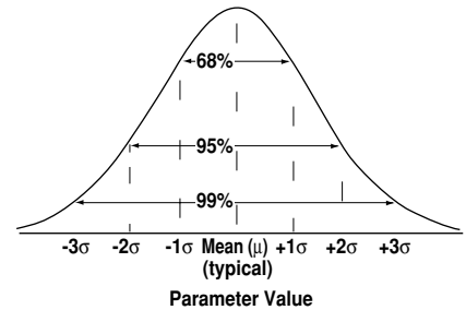
Figure 42. Normal Distribution.
