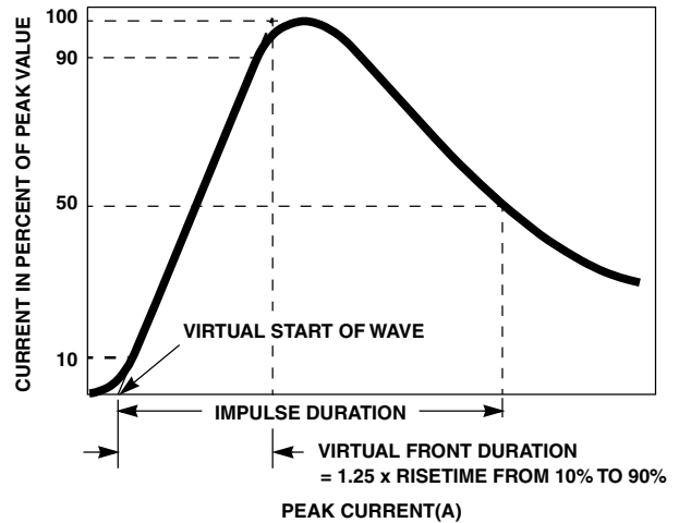
FIGURE 21. DEFINITION OF PULSE CURRENT WAVEFORM
