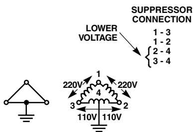
FIGURE 24D. 3 PHASE 220V
